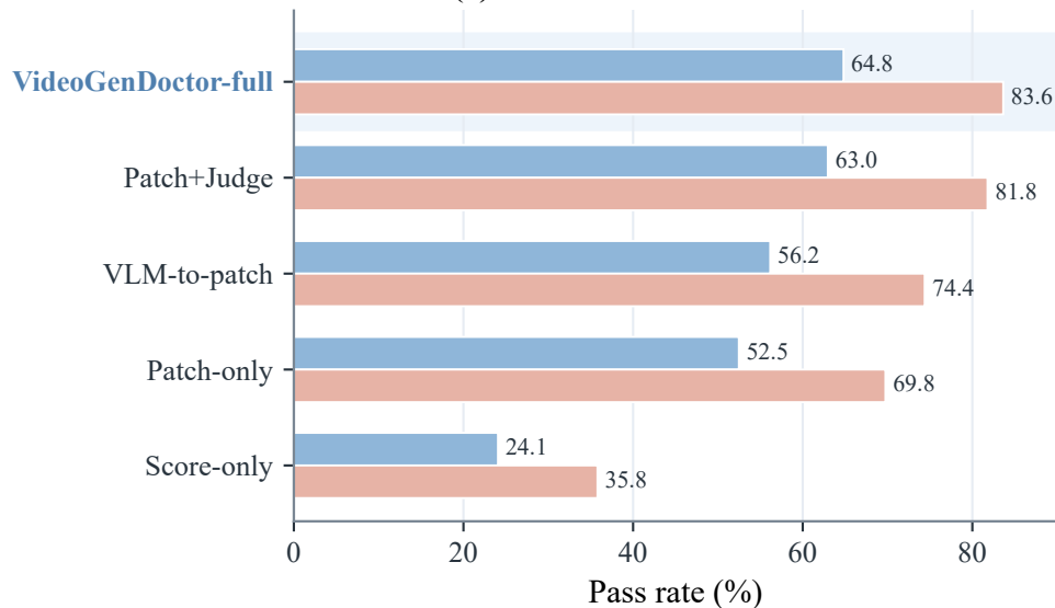
(a) Automatic verifier outcomes
