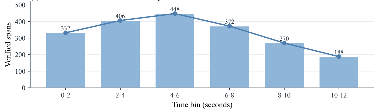
(a) Controlled fixture: 2,016 verified spans
