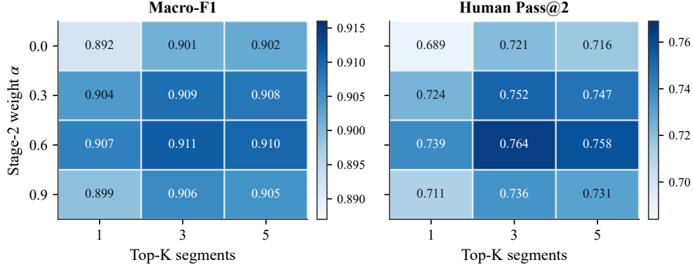
Figure 4: Sensitivity to Stage-2 judge weight \alpha and top- K candidate segments. Each cell reports the draft metric value for a particular (\alpha, K) pair. The default setting, \alpha = 0.6 and K = 3 , yields the strongest balance between diagnosis accuracy and downstream human repair success.
