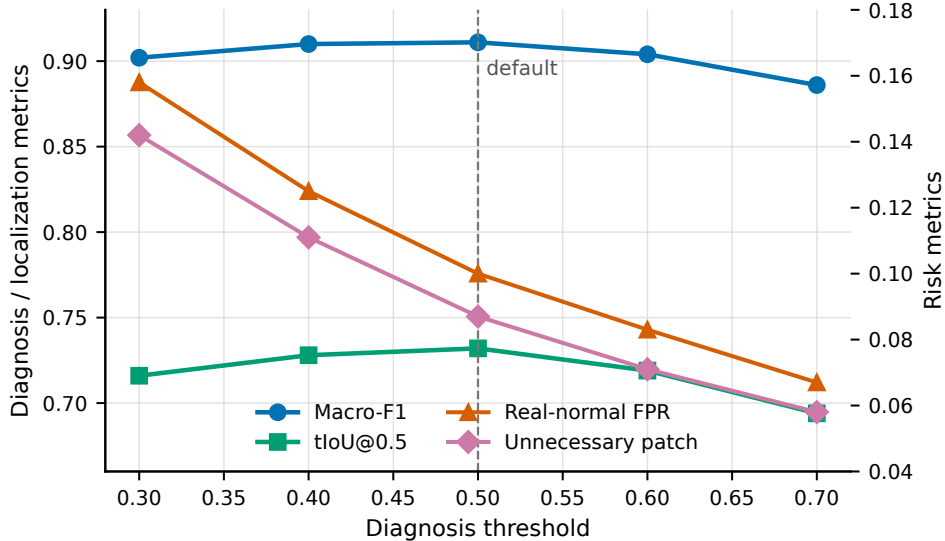
Figure 3: Threshold sensitivity of diagnosis and repair-risk metrics. The default threshold \tau = 0.50 is marked with a vertical dashed line and gives the best diagnosis-localization trade-off, while more conservative thresholds reduce false positives and unnecessary patching.
