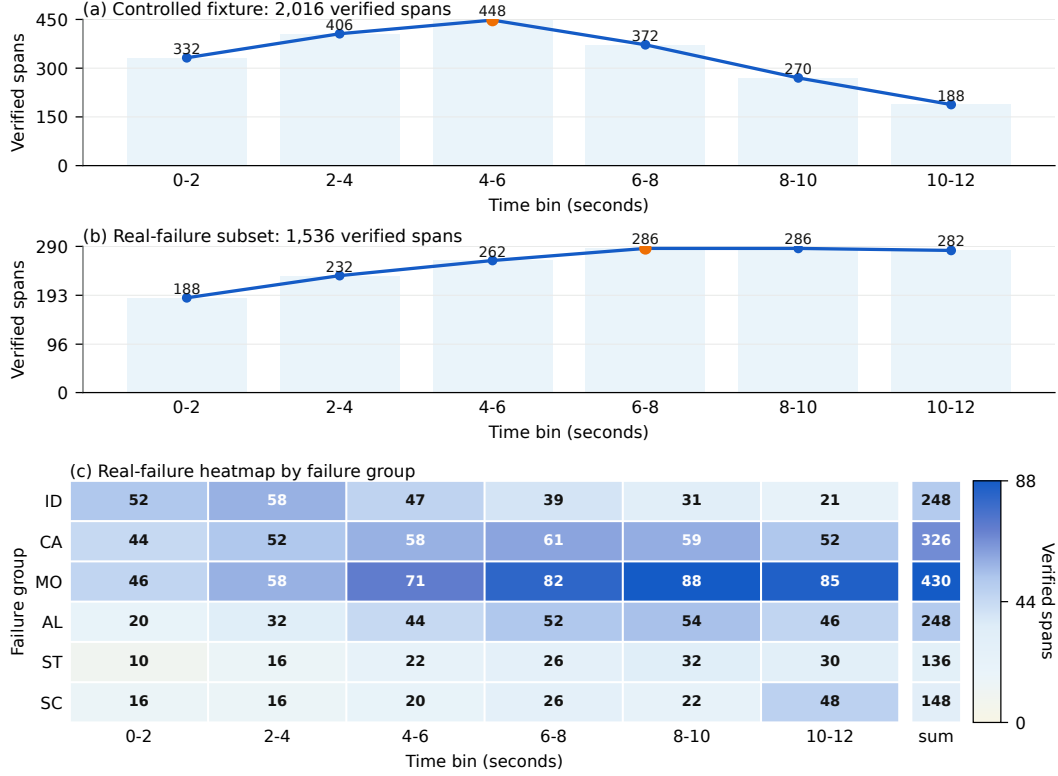
Figure 5: Temporal distribution of verified evidence spans in the evaluation sets. Panel (a) aggregates the 2,016 controlled-fixture spans over 2-second bins and shows the front- and mid-loaded pattern expected from deterministic perturbation operators. Panel (b) summarizes the 1,536 real-failure spans over the same time bins, making the later and more diffuse temporal mass directly comparable to panel (a). Panel (c) further breaks the real-failure spans down by failure group and time bin, highlighting that motion and camera failures dominate the later intervals and overlap more strongly than in the controlled fixture.
