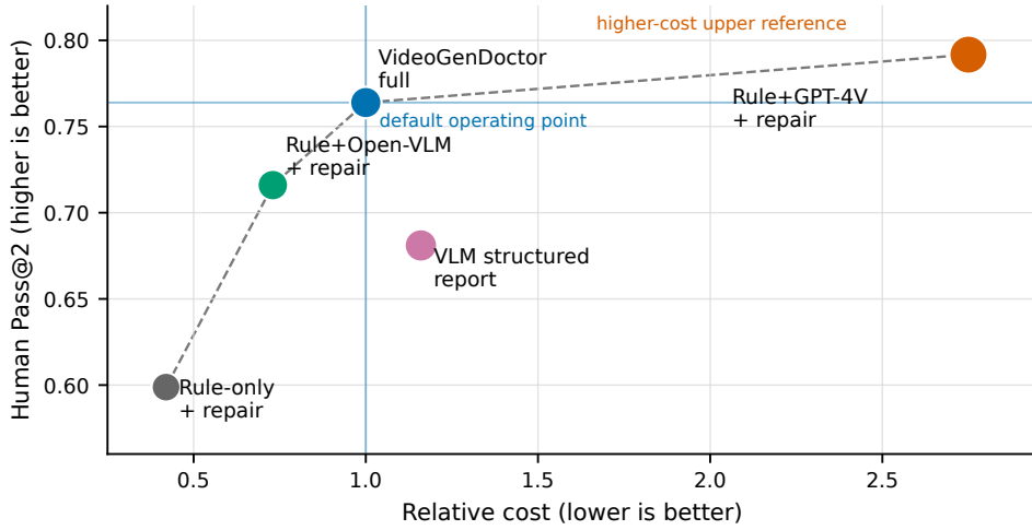
Figure 7: Pareto view of the cost-performance trade-off under the shared downstream repair protocol. The default VideoGenDoctor-full operating point improves human repair success over lower-cost rule variants and direct structured VLM reporting, while the higher-cost Rule+GPT-4V reference obtains the strongest Human Pass@2 at substantially higher relative cost.
