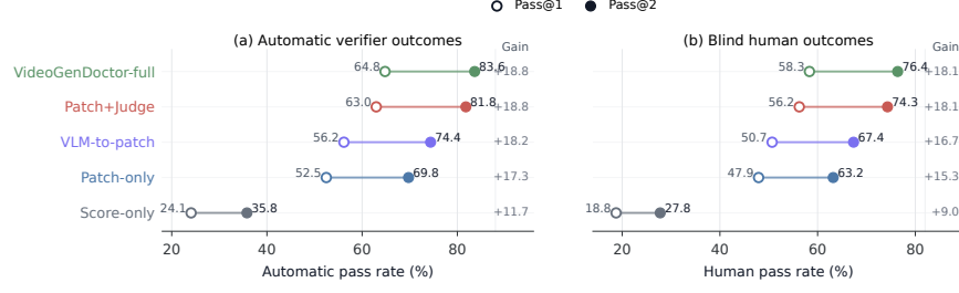
Figure 6: Closed-loop repair comparison on the controlled fixture. Left: automatic verifier Pass@1/2 on all 324 controlled videos. Right: blind human Pass@1/2 on the stratified 144-video human-evaluation subset. Automatic pass rates may be coupled to the system verifier, while human pass rates provide an independent check of repair success.
