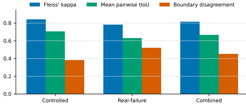
Figure 10: Draft multi-annotator stability analysis. Code-level Fleiss' \kappa is higher than temporal-boundary agreement, and the real-failure subset remains the most ambiguous split.
