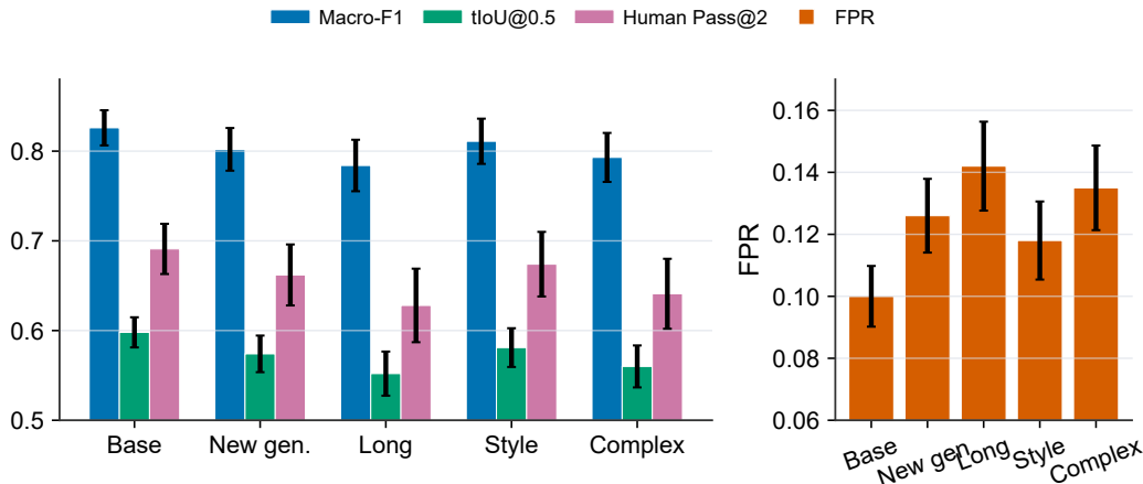
Figure 9: Draft stress validation on harder real-failure slices. Left: diagnosis, localization, and human repair metrics with uncertainty bars. Right: false-positive rate on matched real-normal controls for each slice.
