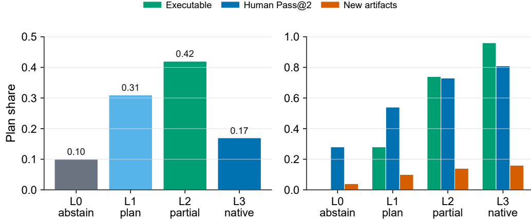
Figure 8: Adapter-executability stratification by repair-plan level. The left panel reports the share of generated plans by adapter level; the right panel compares adapter-executable rate, Human Pass@2, and new-artifact rate within each level.
