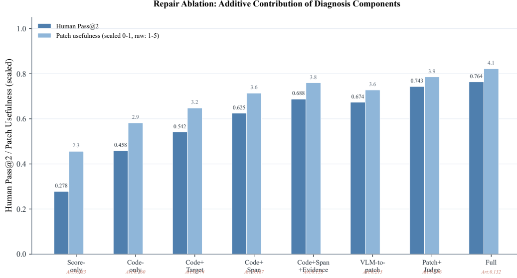
Figure 5: Repair ablation as grouped bars. Human Pass@2 (dark blue) and patch usefulness (light blue, scaled) rise additively as code, span, evidence, and verification are incorporated. New-artifact rates (annotated at bottom) trend downward as diagnosis quality improves.
