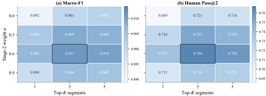
Figure 7: Sensitivity to judge weight \alpha and candidate budget K . \alpha = 0.6 , K = 3 balances diagnosis accuracy and repair success; \alpha = 0.9 introduces instability from VLM over-correction.
