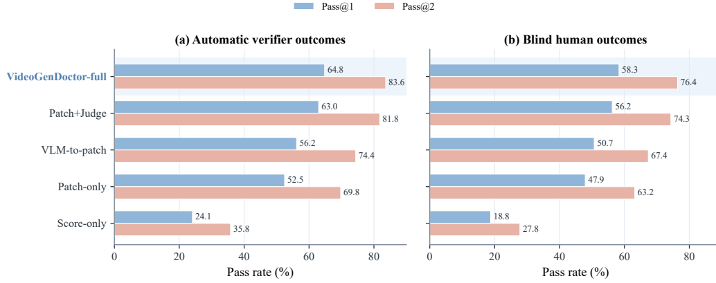
Figure 9: Closed-loop repair comparison on the controlled fixture. Left: automatic verifier Pass@1/2 on all 324 controlled videos. Right: blind human Pass@1/2 on the stratified 144-video human-evaluation subset. Automatic pass rates may be coupled to the system verifier, while human pass rates provide an independent check of repair success.
