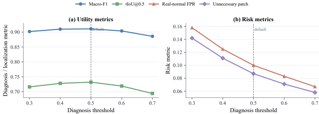
Figure 6: Threshold sensitivity curves. Dashed line at \tau = 0.50 marks the operating point where macro-F1 and tIoU@0.5 peak before false positives rise sharply.
