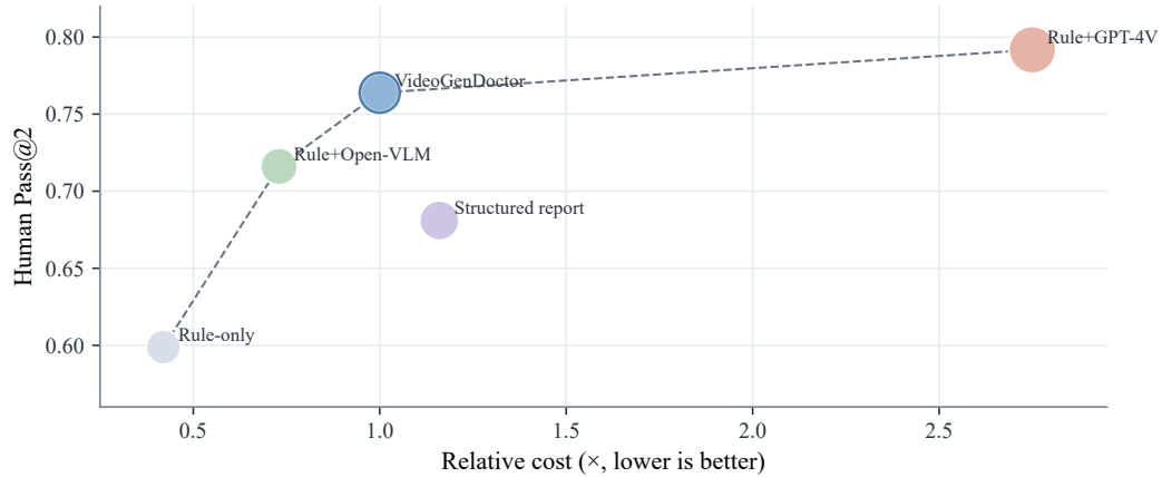
Figure 10: Pareto view of the cost-performance trade-off under the shared downstream repair protocol. The default VideoGenDoctor-full operating point improves human repair success over lower-cost rule variants and direct structured VLM reporting, while the higher-cost Rule+GPT-4V reference obtains the strongest Human Pass@2 at substantially higher relative cost.
