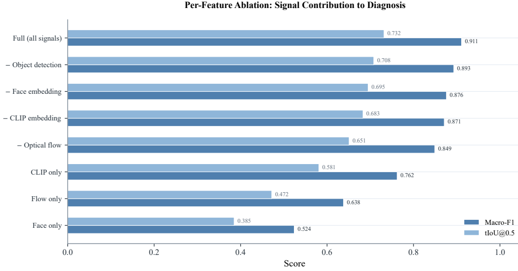
Figure 4: Per-feature ablation. Optical flow is the single most critical signal; single-signal configurations (bottom three rows) all underperform substantially, confirming complementary contributions.
