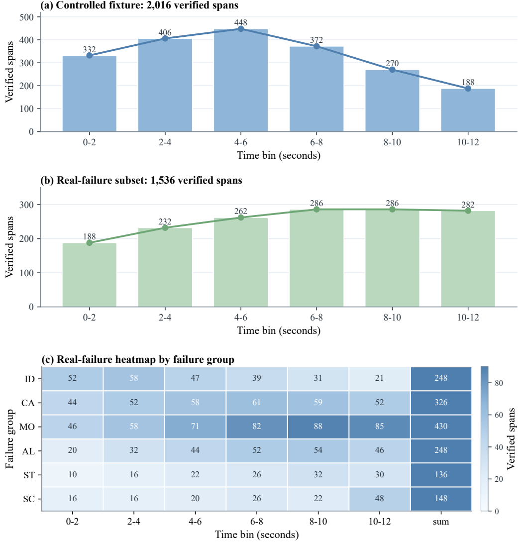
Figure 8: Temporal distribution of verified evidence spans in the evaluation sets. Panel (a) aggregates the 2,016 controlled-fixture spans over 2-second bins and shows the front- and mid-loaded pattern expected from deterministic perturbation operators. Panel (b) summarizes the 1,536 real-failure spans over the same time bins, making the later and more diffuse temporal mass directly comparable to panel (a). Panel (c) further breaks the real-failure spans down by failure group and time bin, highlighting that motion and camera failures dominate the later intervals and overlap more strongly than in the controlled fixture.
