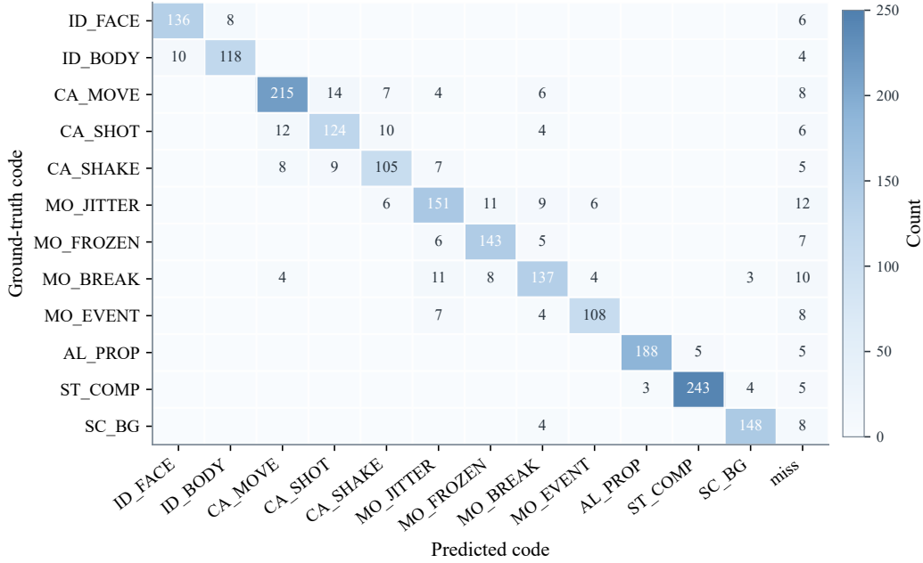
Figure 2: Per-code confusion matrix on the controlled fixture. Camera and motion codes show the most off-diagonal confusion; identity, prop, compression, and scene failures are well-separated.
