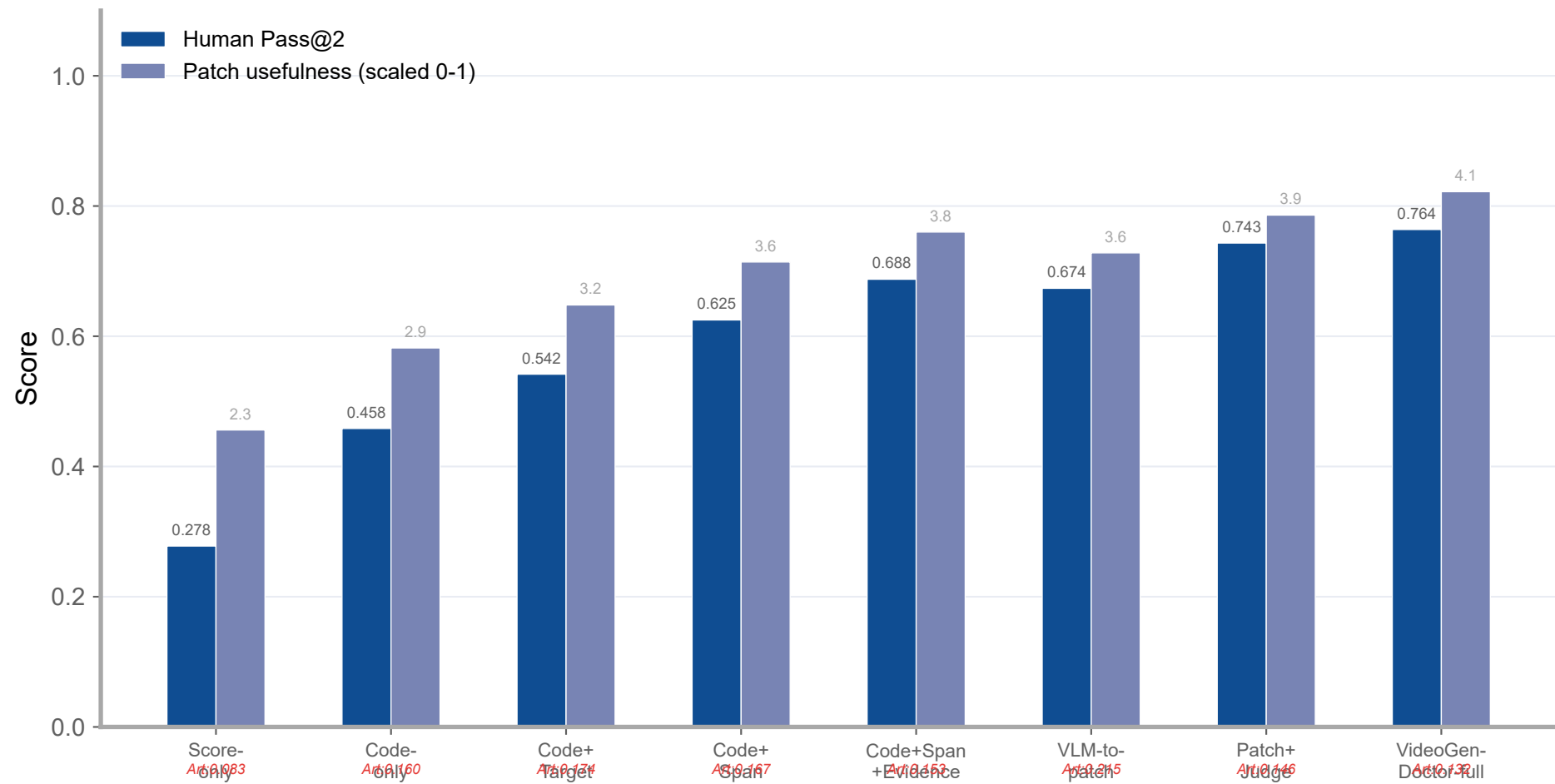
Repair ablation: additive contribution of diagnosis components
