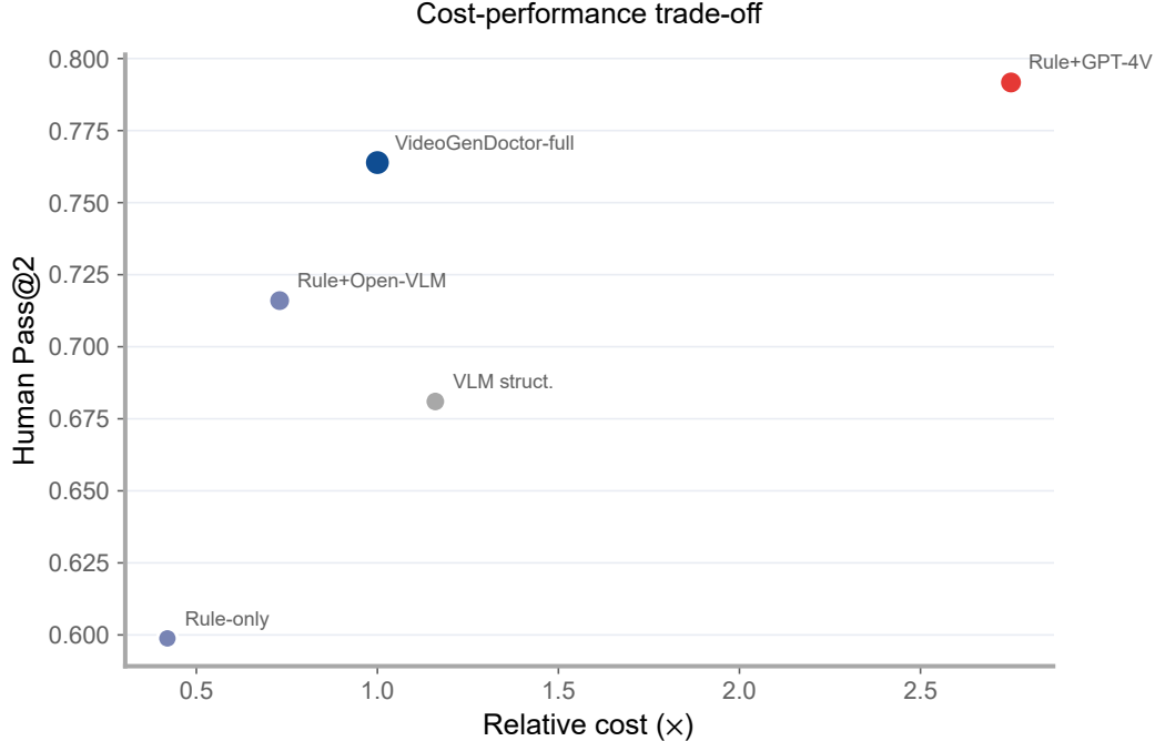
Figure 4: Pareto view of the cost-performance trade-off under the shared downstream repair protocol. The default VideoGenDoctor-full operating point improves human repair success over lower-cost rule variants and direct structured VLM reporting, while the higher-cost Rule+GPT-4V reference obtains the strongest Human Pass@2 at substantially higher relative cost.
