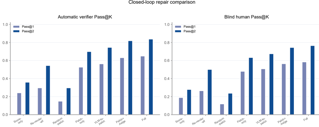
Figure 3: Closed-loop repair comparison on the controlled fixture. Left: automatic verifier Pass@1/2 on all 324 controlled videos. Right: blind human Pass@1/2 on the stratified 144-video human-evaluation subset. Automatic pass rates may be coupled to the system verifier, while human pass rates provide an independent check of repair success.
