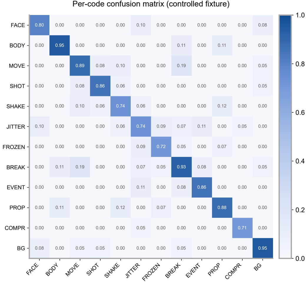
Figure 5: Per-code confusion matrix on the controlled fixture. Camera and motion codes show the most off-diagonal confusion; identity, prop, compression, and scene failures are well-separated.
