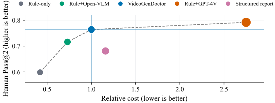
Figure 7: Pareto view of the cost-performance trade-off under the shared downstream repair protocol. The default VideoGenDoctor-full operating point improves human repair success over lower-cost rule variants and direct structured VLM reporting, while the higher-cost Rule+GPT-4V reference obtains the strongest Human Pass@2 at substantially higher relative cost.
