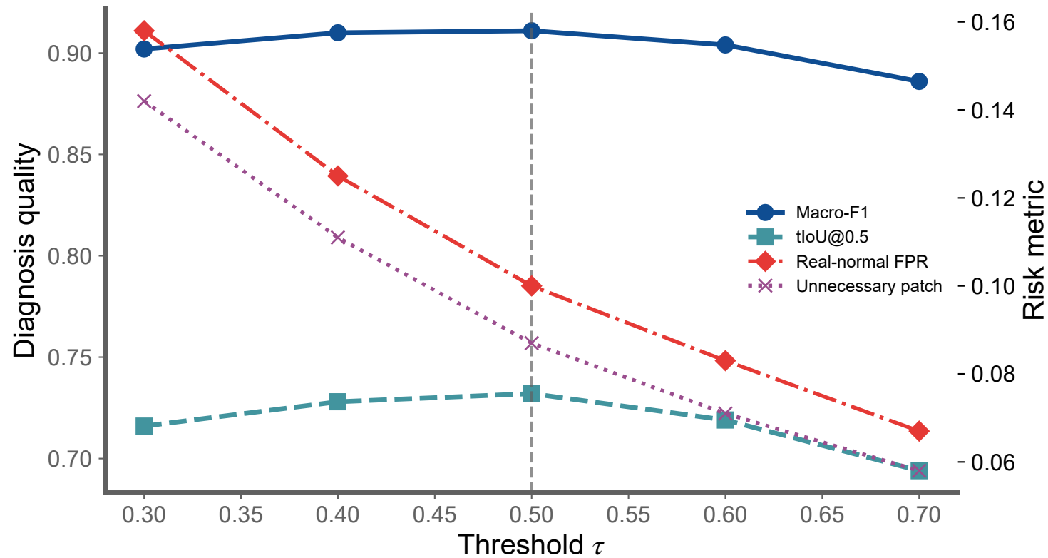
Threshold sensitivity
