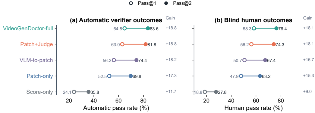
Figure 6: Closed-loop repair comparison on the controlled fixture. Left: automatic verifier Pass@1/2 on all 324 controlled videos. Right: blind human Pass@1/2 on the stratified 144-video human-evaluation subset. Automatic pass rates may be coupled to the system verifier, while human pass rates provide an independent check of repair success.
