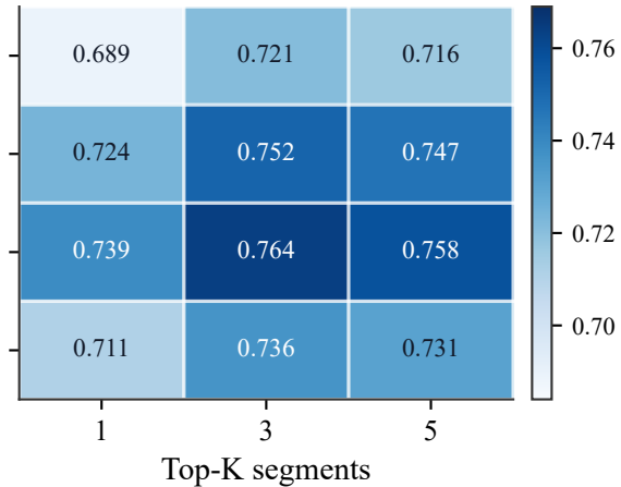
Human Pass@2
