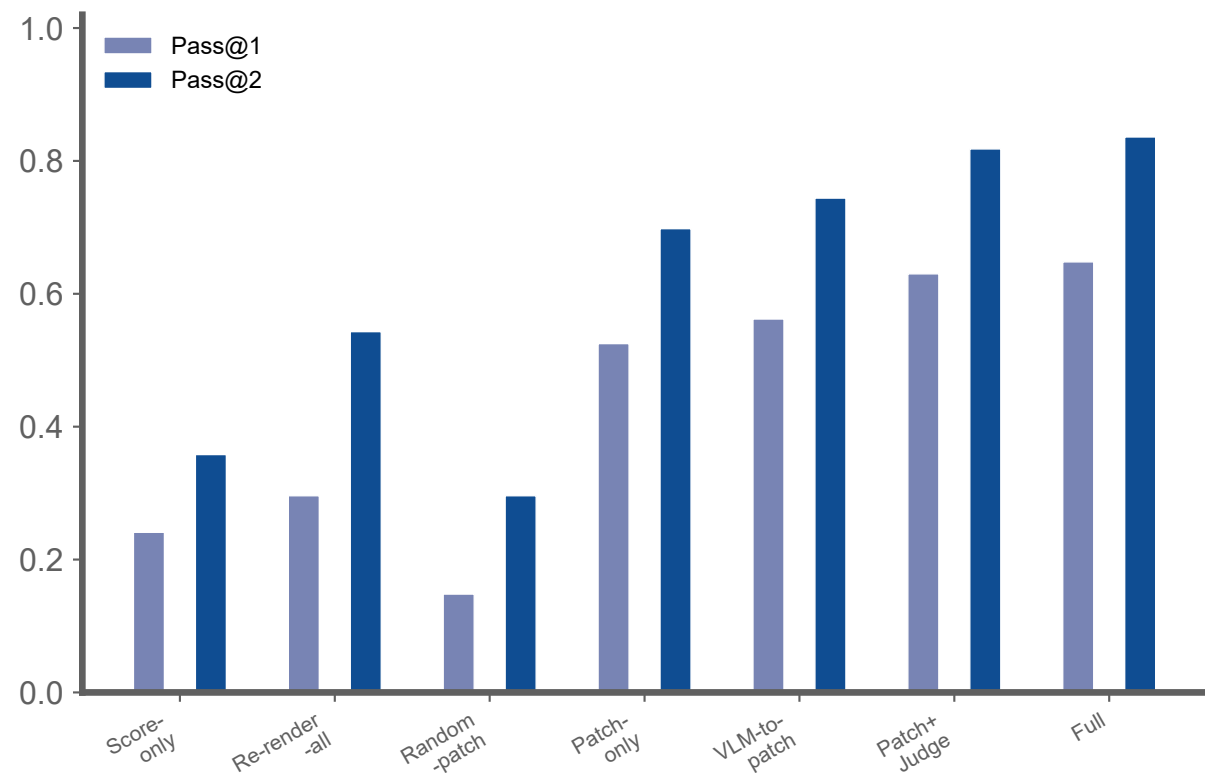
Automatic verifier Pass@K
