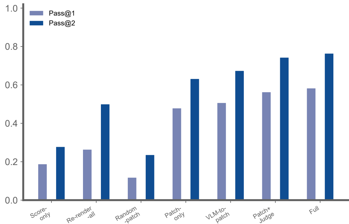
Blind human Pass@K
