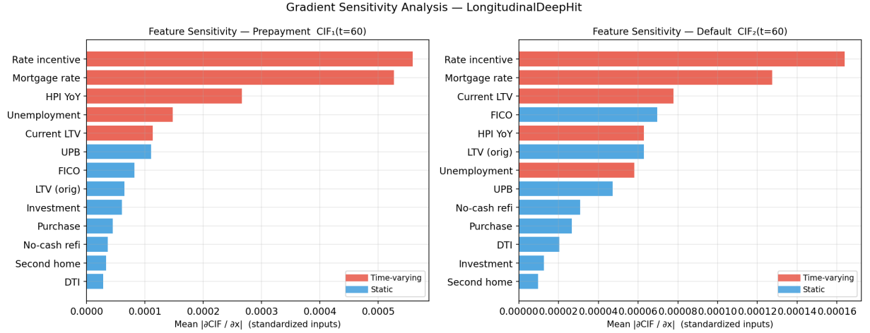
Figure 3: Mean |\partial CIF / \partial x| over 500 test loans and all timesteps. Left: prepayment CIF_1 at month 60. Right: default CIF_2 at month 60. Red: time-varying features. Blue: static features.
