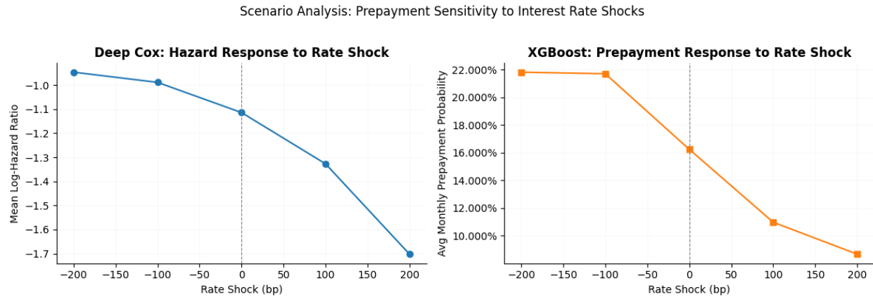
Fig 8. Prepayment sensitivity to interest rate shocks. XGBoost (right) shows clear monotone convex response; Deep Cox (left) shows a smoother log-hazard ratio response.
