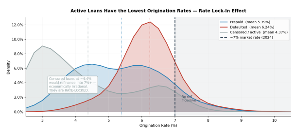
Fig 3 (left). LTV equity trap: 37% of defaults vs 23% of prepayments are above the 80% LTV conventional refi threshold — high LTV removes the escape valve. Fig 4 (right). Rate lock-in: active loans originated at ~4.4% cannot refinance into 7%+ market rates — this is the dominant driver of suppressed prepayment post-2022.
