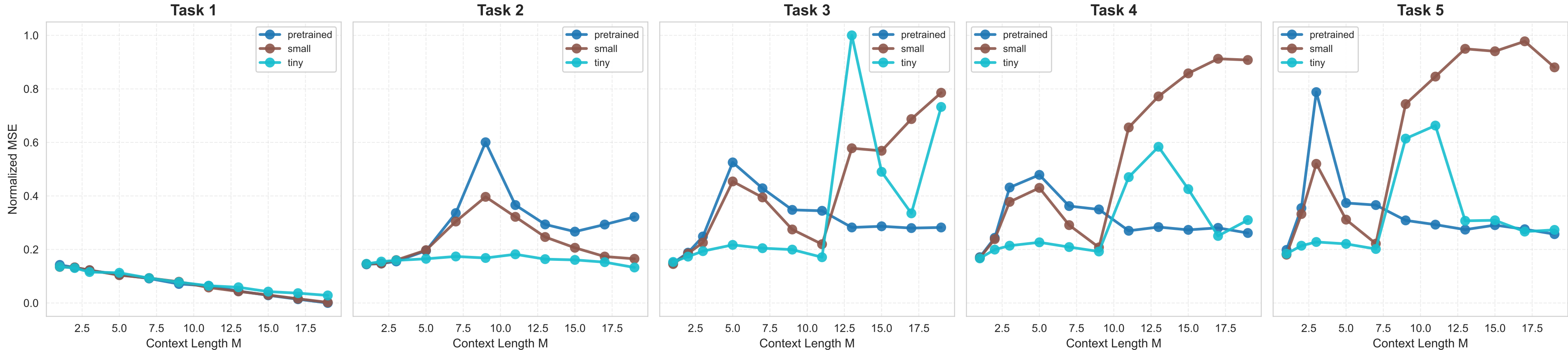
Per-task MSE vs M (multi-model)
