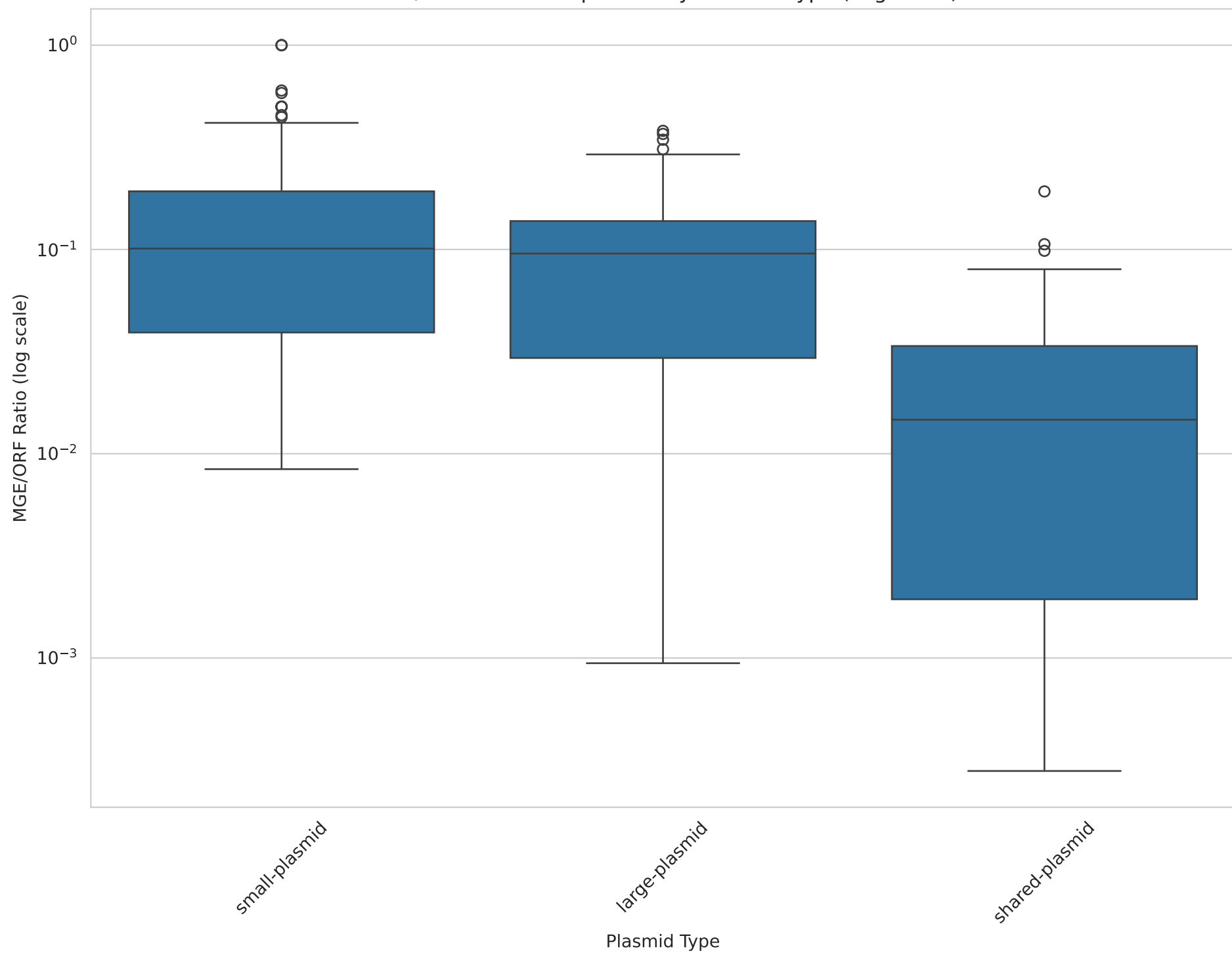
MGE/ORF Ratio Comparison by Plasmid Type (Log Scale)
