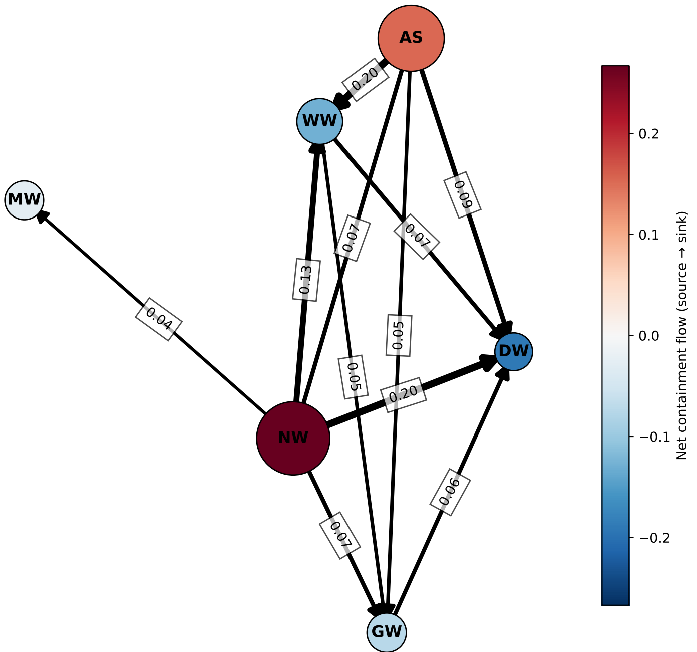
Global directional flow of clusters among environments
