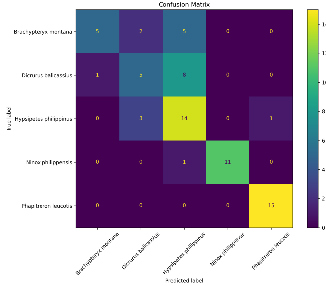
Fig. 7. Confusion matrix of the final model on the held-out test set.
