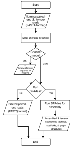
Fig. 4: MitoChime pipeline for model selection, filtering, and optional assembly evaluation.
