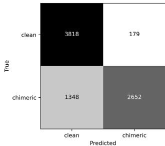
Gradient Boosting
