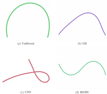
Figure F.7: Assembly graphs for 10K paired-end reads at 15% chimera proportion.
