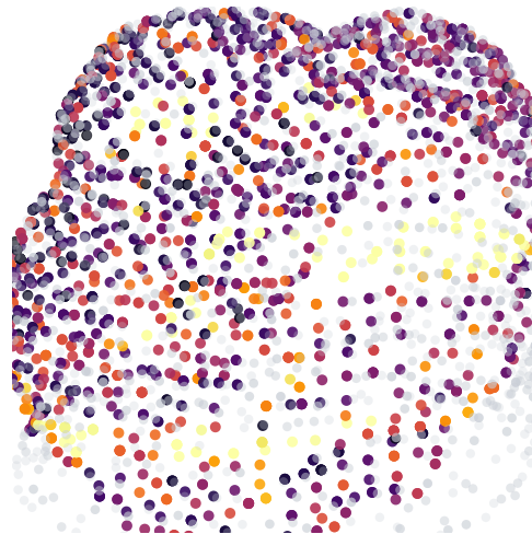
Prediction error
