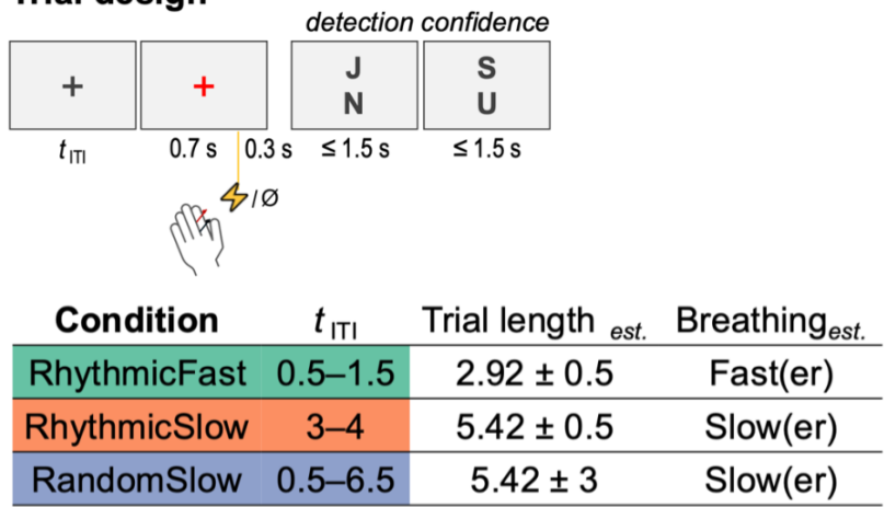
Figure 1. Experimental design of respirationAdj1 (3 conditions; rhythmic fast = RhyF, rhythmic slow = RhyS, random slow = RanS). Estimated (est.) trial length equals the mean ITI, time window of the red fixation cross (1 s), and grand median detection and confidence RTs from Forster et al. (2025, Exp 2). Blocks consist of 80 trials (RhyS, RanS) or 160 trials (RhyF) to approximate similarity in duration. At the beginning of each block, starting periods are implemented that last about 30 s with ITIs matching the mean ITI of the respective other faster or slower condition (RhyF blocks: 6 trials with t_{\text{Starting ITI}} of 3.5 s; RhyS and RanS blocks: 10 trials with t_{\text{Starting ITI}} of 1 s). Excluding those starting period trials, the total trial count per condition is 320 trials (voltage symbol: 240 signal-present; empty set symbol: 80 signal-absent). Offline threshold assessments are used (and repeated prior to each block) to identify individual near-threshold intensities (mA) of approximately 60% detectability (similar procedure as in Forster et al., 2025; Grund et al., 2022). Near-threshold signals are delivered to the left index finger; button responses are given with the right index finger.
