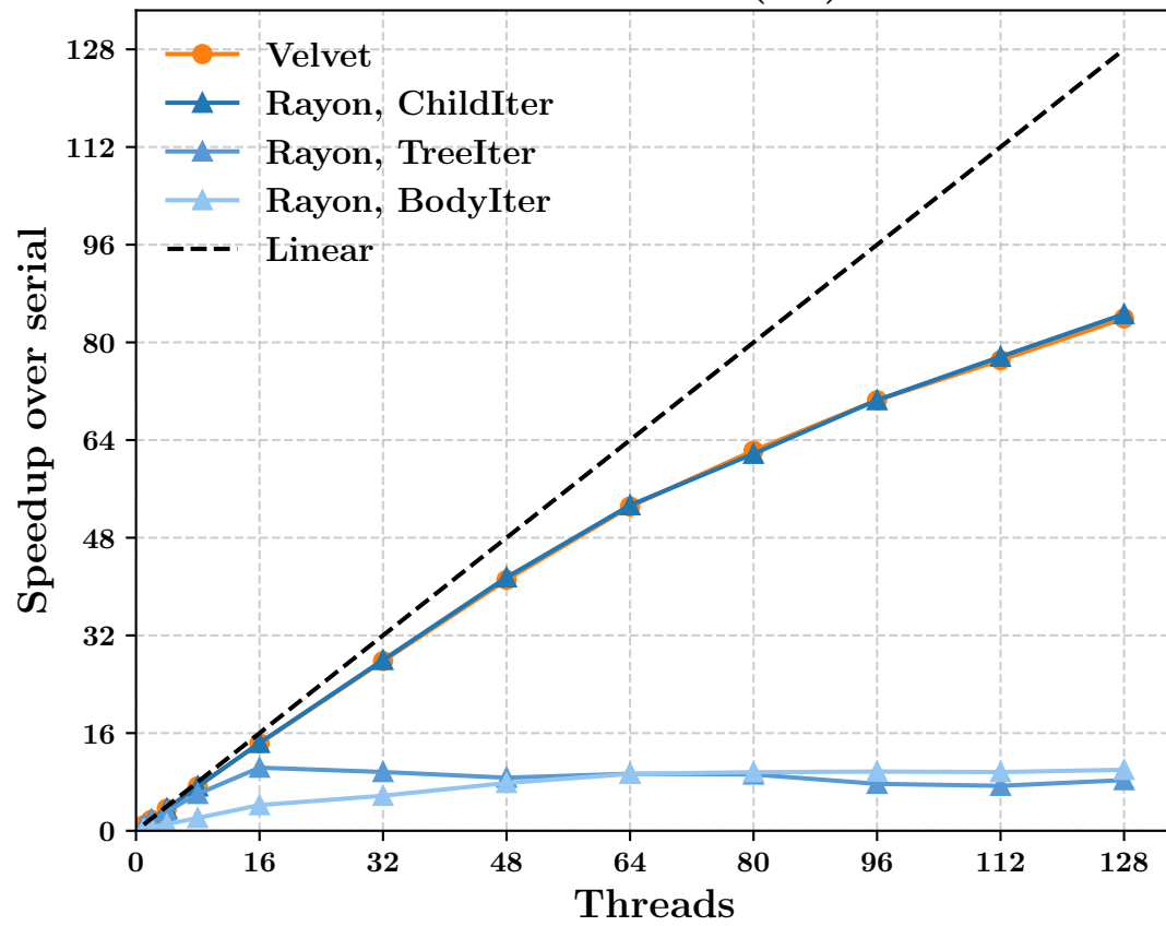
Barnes-Hut ( bh )
