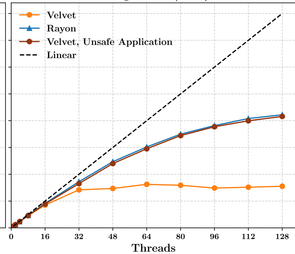
Merge Sort ( sort )
