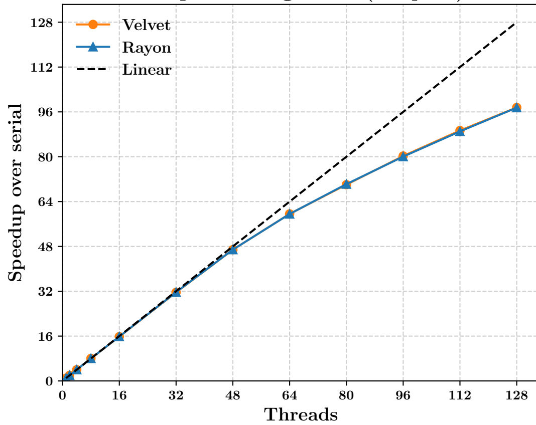
Adaptive Integration ( adapint )
