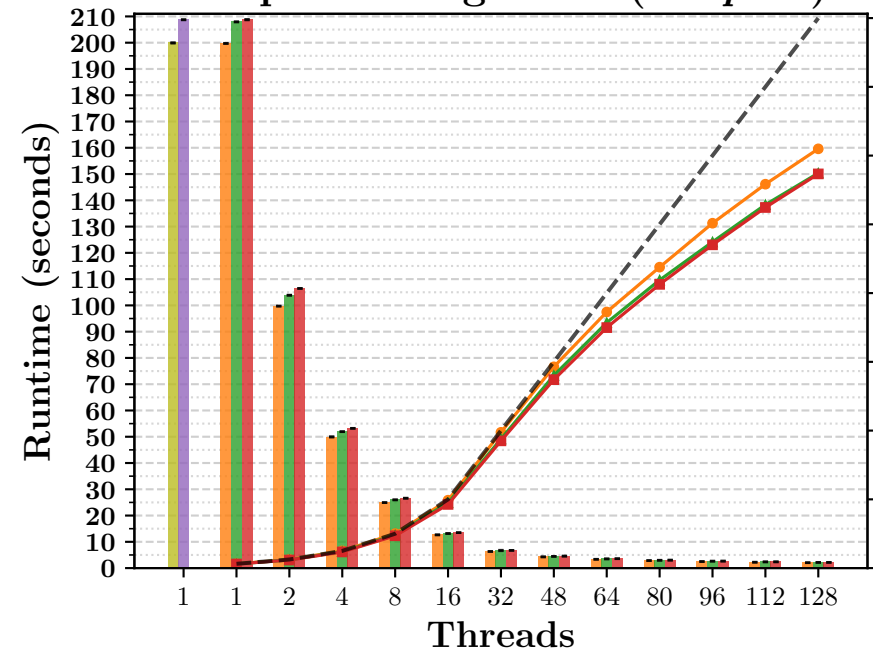
Barnes-Hut ( bh )
