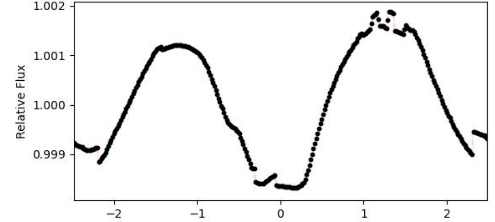
Transit-view weak secondary flux N_transits=5
