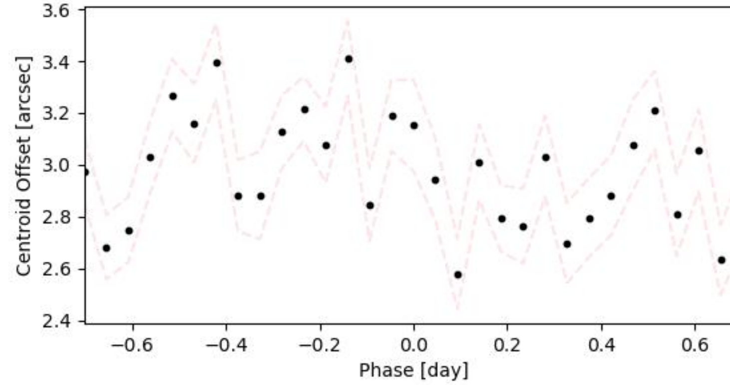
Transit-view centroid offset to target N_transits=5
