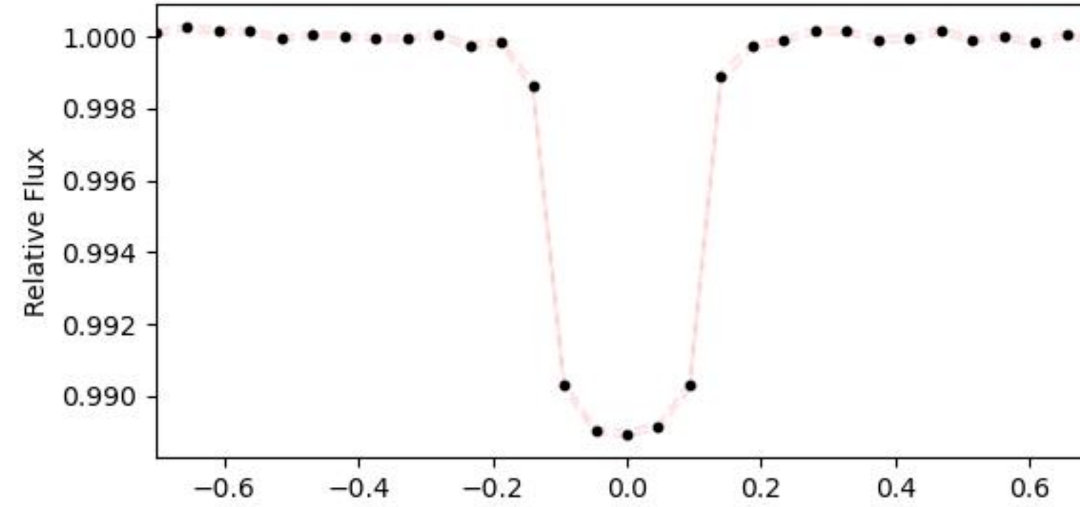
Transit-view even flux N_transits=3
