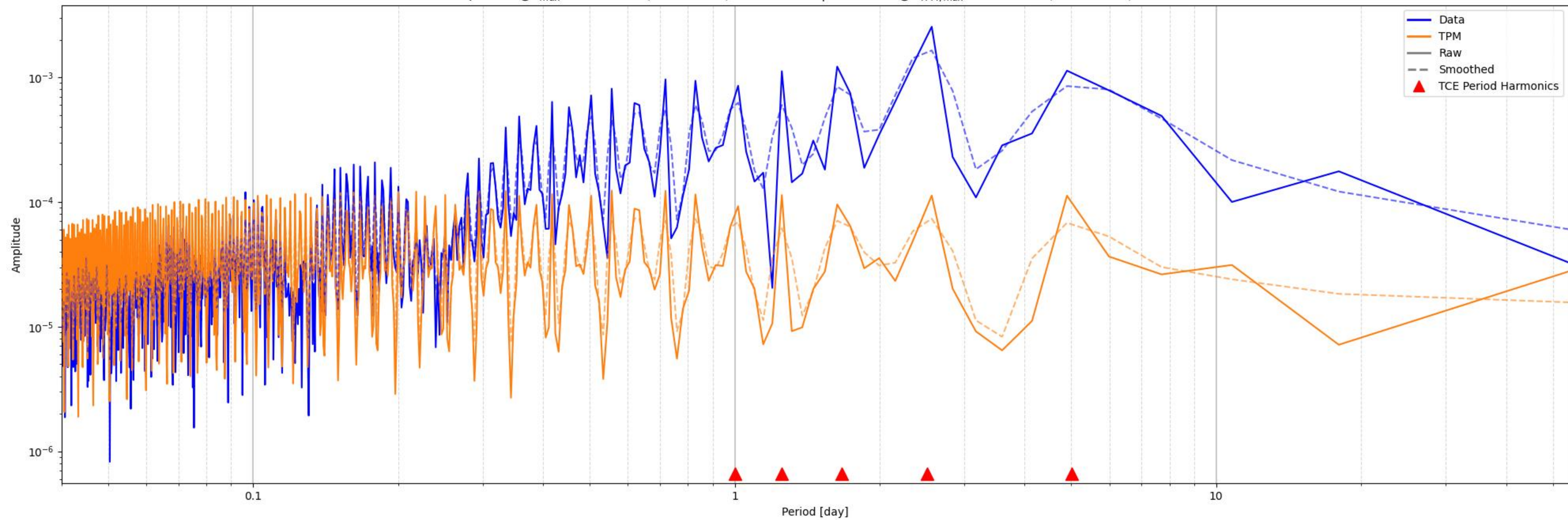
Periodogram TCE 167526485-1-S6 | Period: 5.012 day Peak Amplitude @ f_{max} = 0.390 \text{ d}^{-1} ( P = 2.566 \text{ d} ): 2.548e-03 | TPM Peak @ f_{TPM,max} = 1.800 \text{ d}^{-1} ( P = 0.555 \text{ d} ): 1.235e-04
