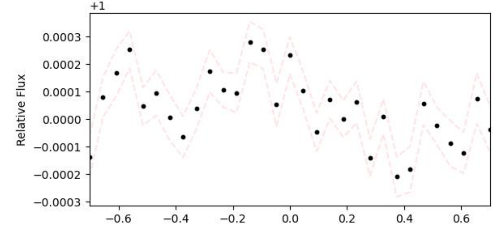
Transit-view weak secondary flux N_transits=5
