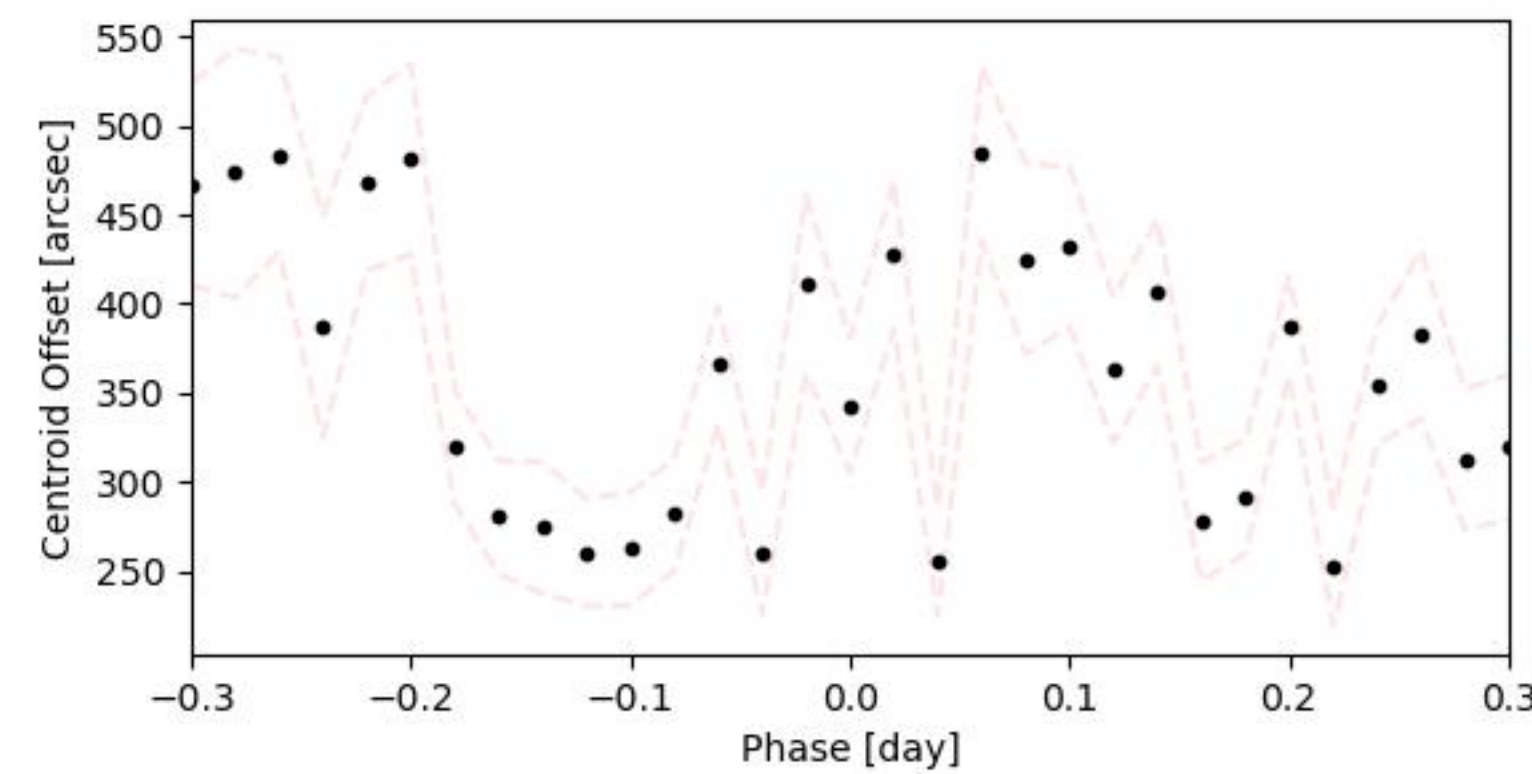
Transit-view centroid offset to target N_transits=5
