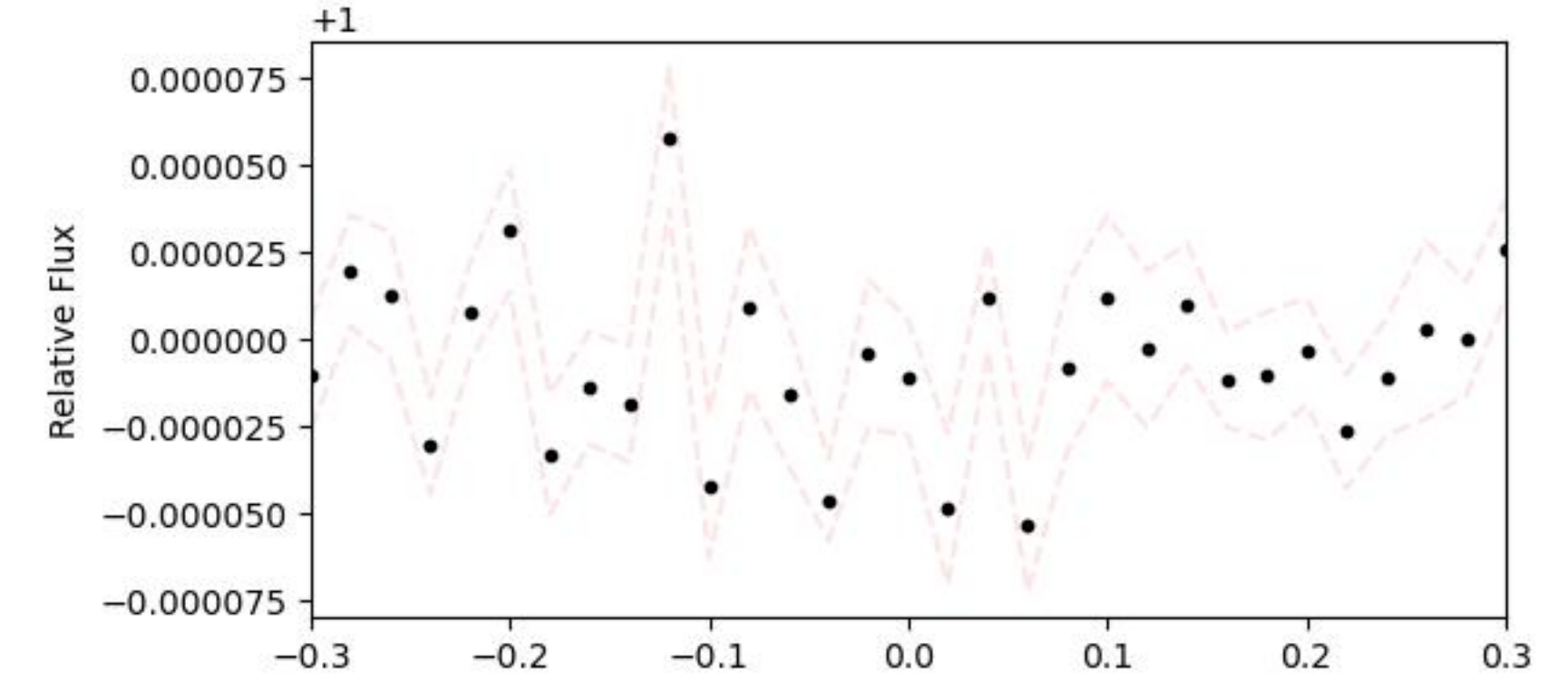
Transit-view weak secondary flux N_transits=6
