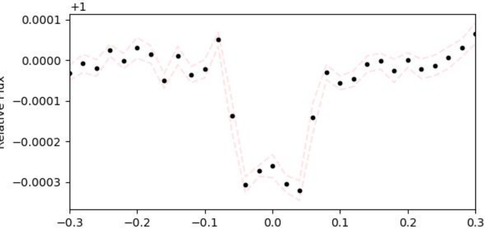
Transit-view odd flux N_transits=2
