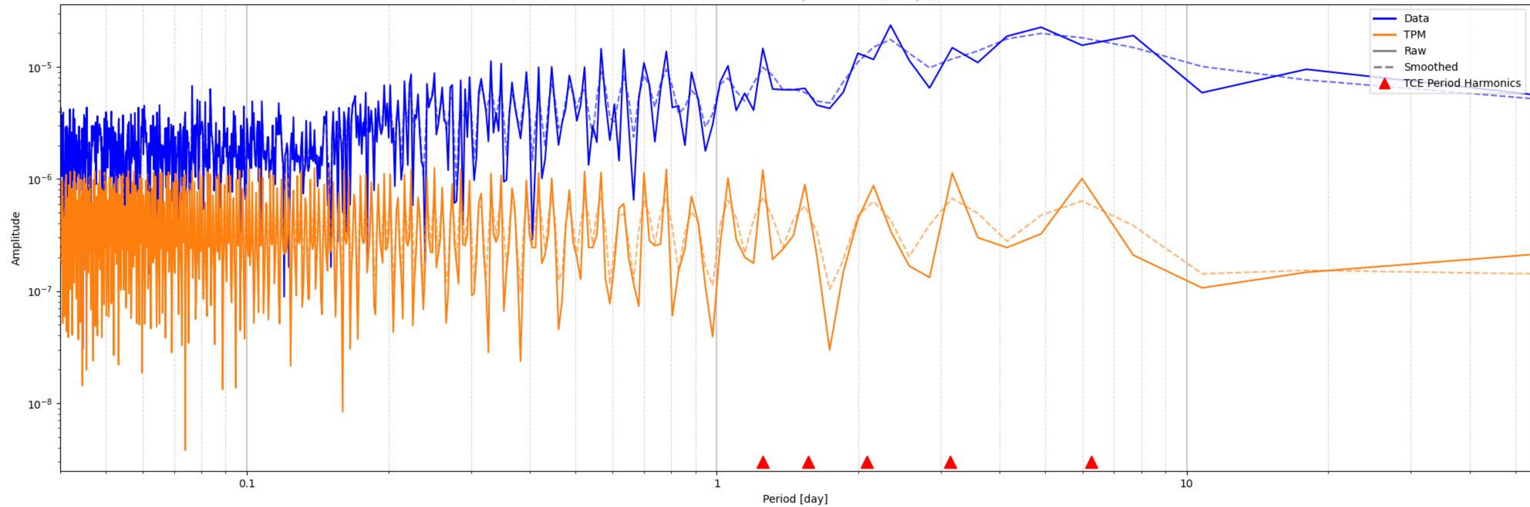
Periodogram TCE 261136679-1-S1 | Period: 6.267 day Peak Amplitude @ f_{max} = 0.427 \text{ d}^{-1} ( P = 2.343 \text{ d} ): 2.352e-05 | TPM Peak @ f_{TPM,max} = 3.990 \text{ d}^{-1} ( P = 0.251 \text{ d} ): 1.258e-06
