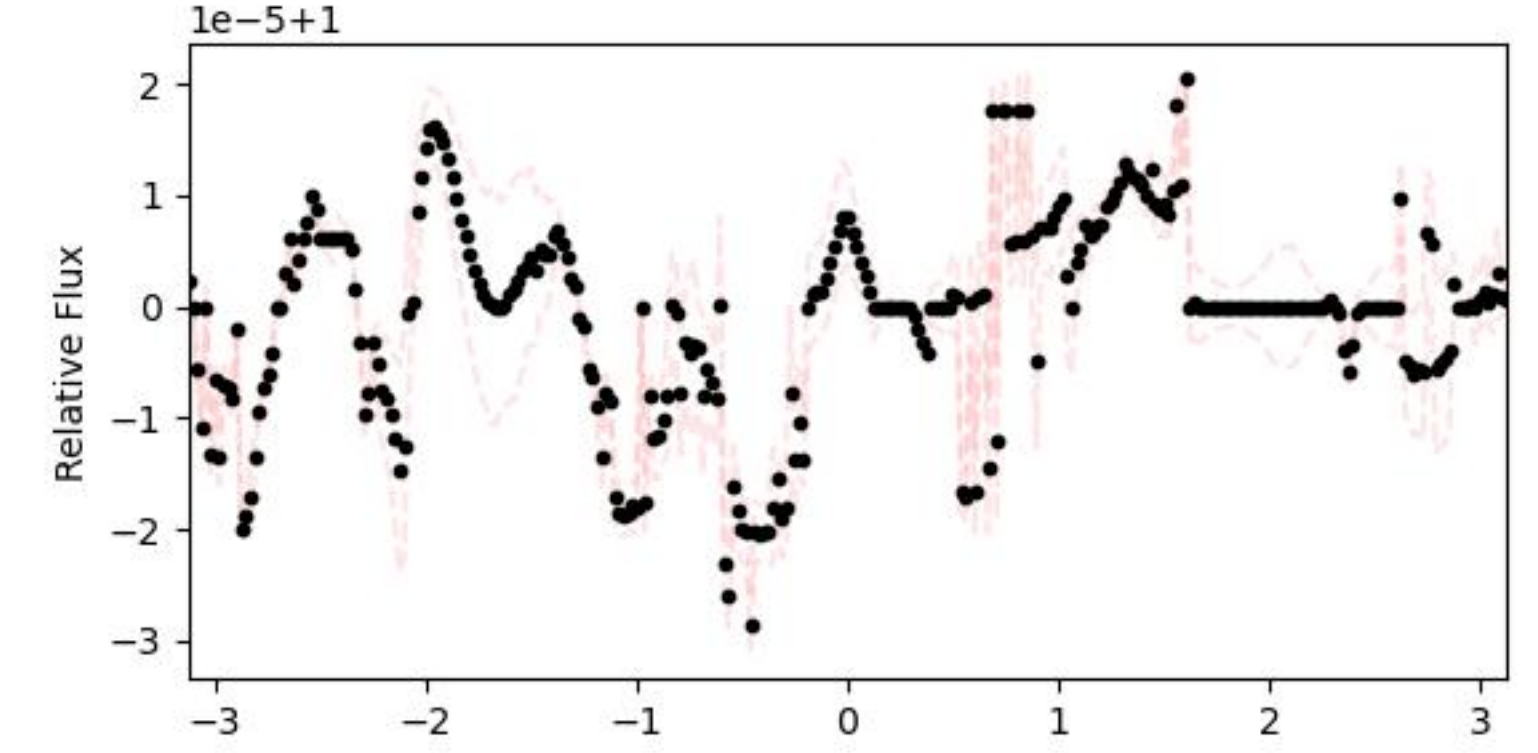
Full-orbit trend N_transits=5
