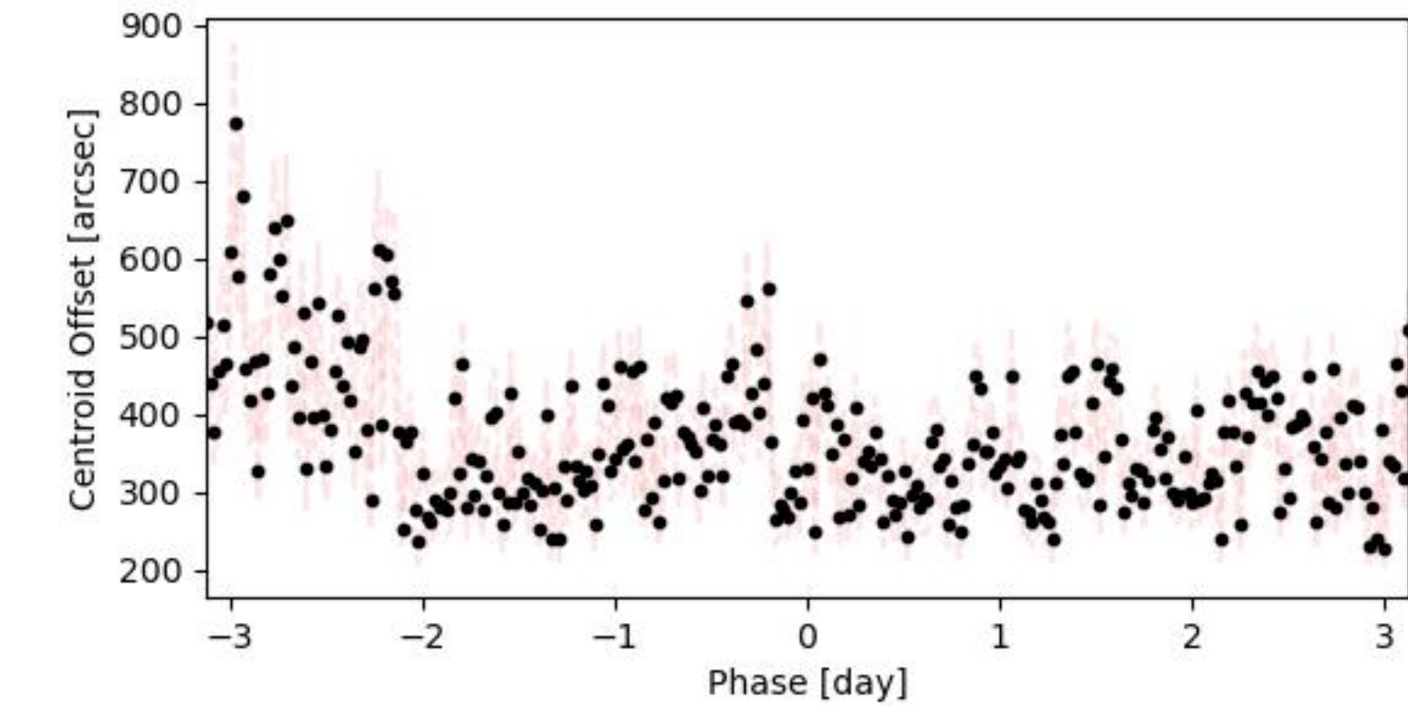
Full-orbit centroid offset to target N_transits=5
