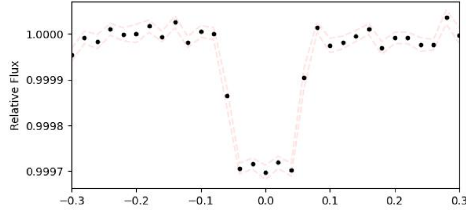
Transit-view even flux N_transits=3
