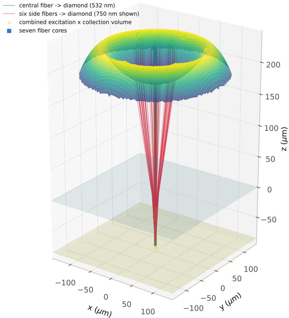
(a) Rays propagate from fibers into diamond
