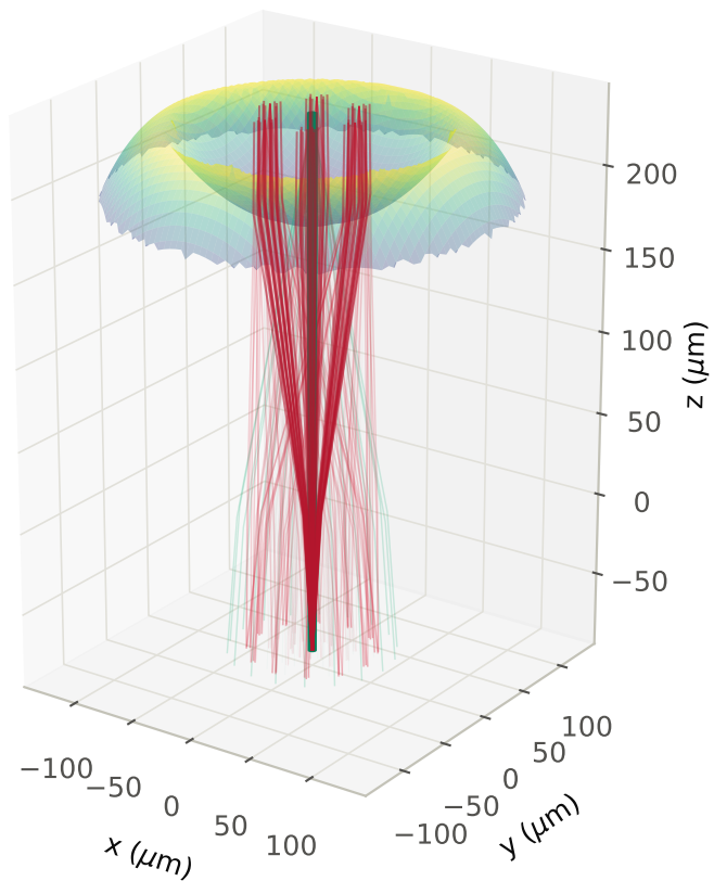
(a) Full-NA envelopes of all seven cores
