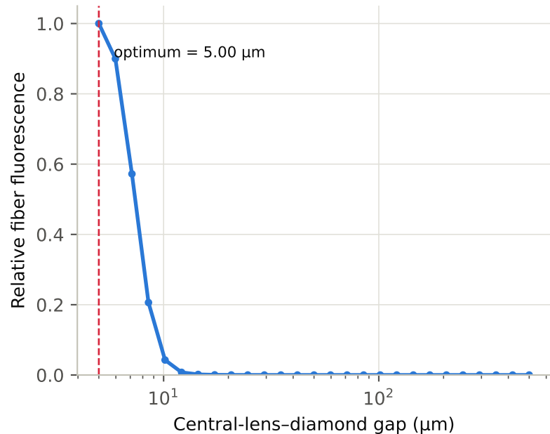
(a) Fixed printed tip: Z-distance sweep
