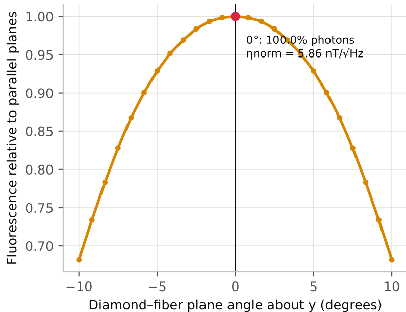
(b) Angular misalignment at optimum Z
