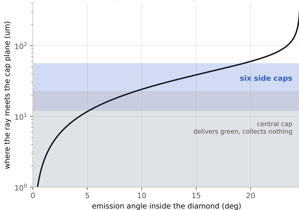
(b) so the caps are placed where that light lands
