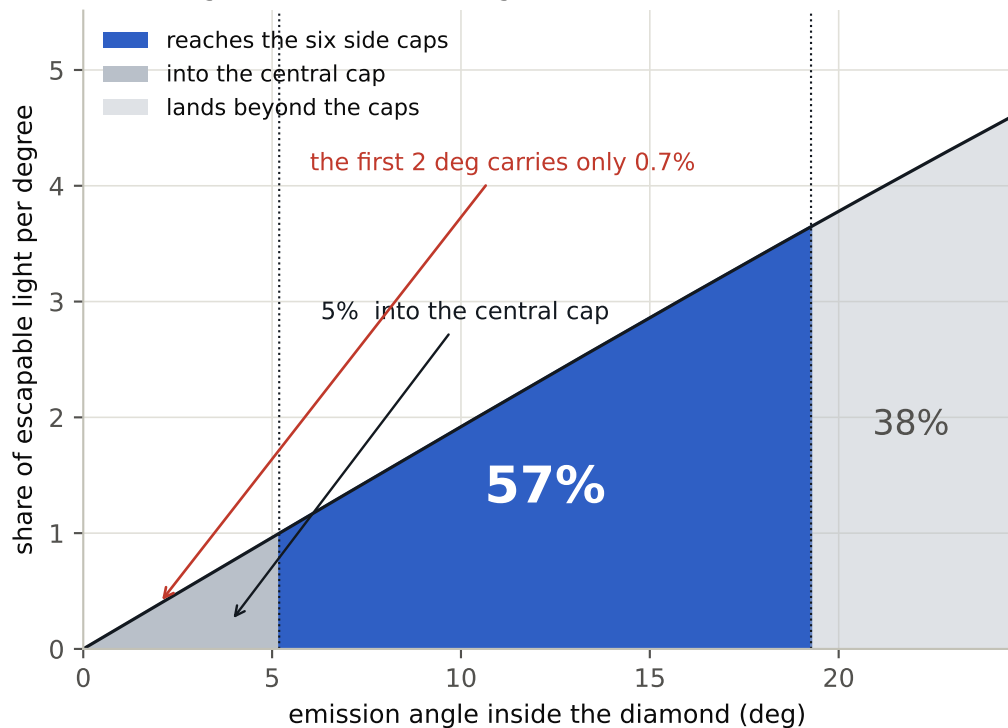
(a) the light is in the outer angles, not near the axis
