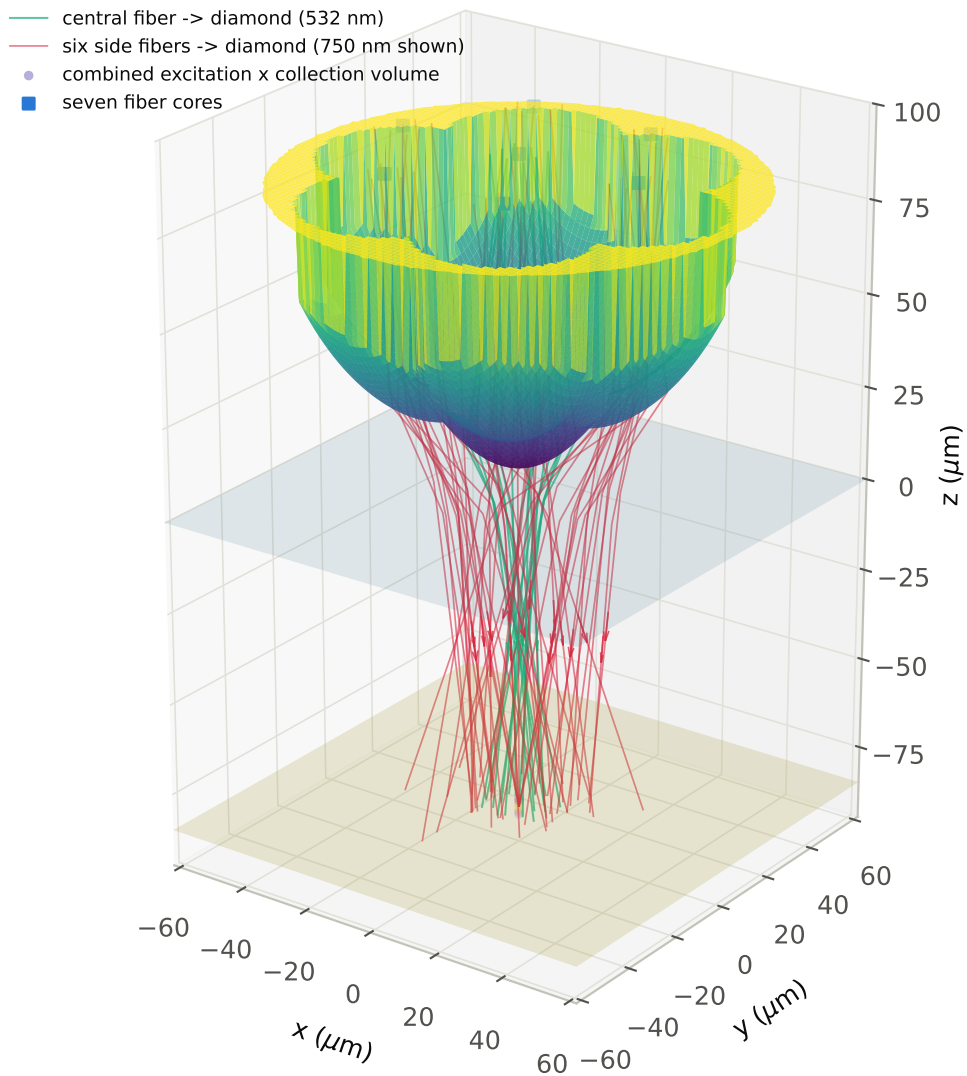
(a) Rays propagate from fibers into diamond
