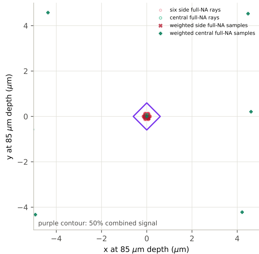
(c) Full-NA landing positions and scored overlap
