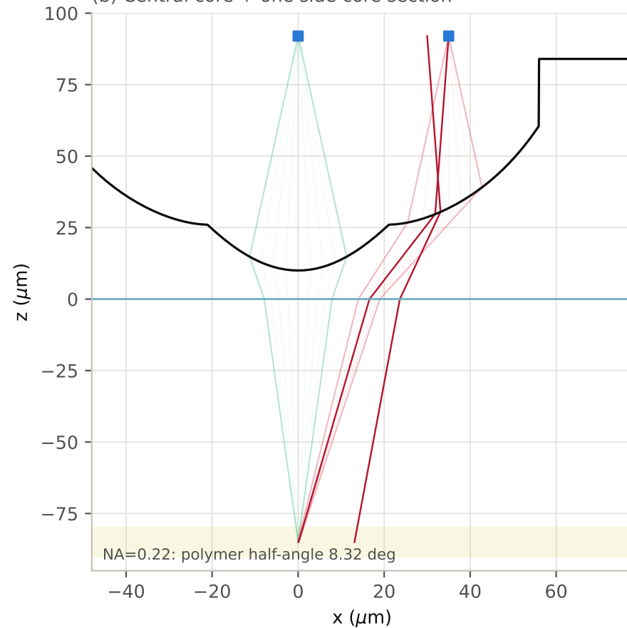
(b) Central core + one side core section
