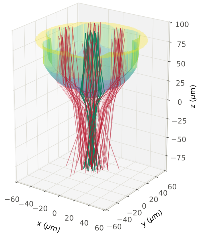
(a) Full-NA envelopes of all seven cores
