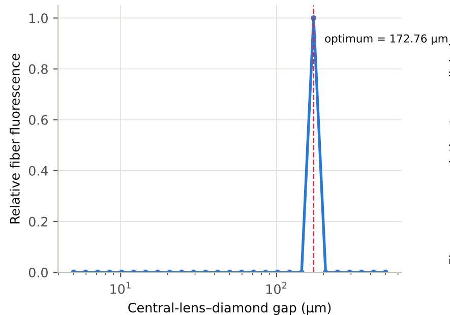
(a) Fixed printed tip: Z-distance sweep
