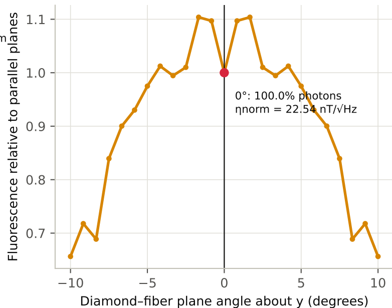
(b) Angular misalignment at optimum Z
