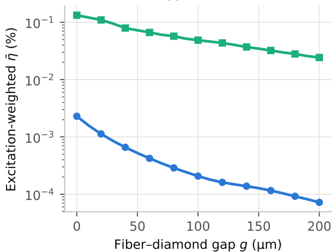
(c) ensemble, 3 ppm
