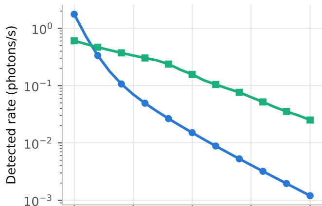
(b) single NV, 10 mW exc.
