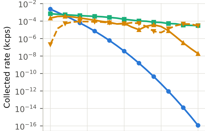
(b) single NV, 10 mW excitation
