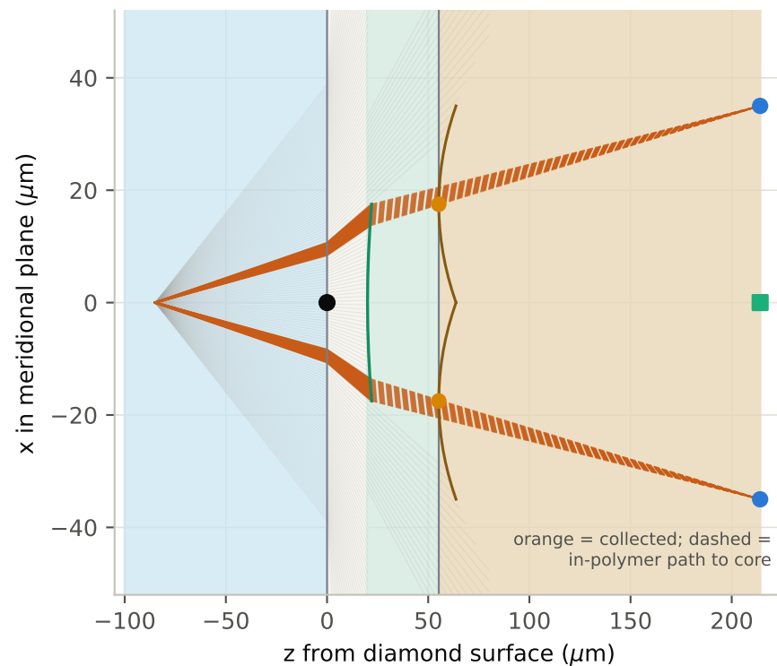
(c) 700 nm rays at fixed-design optimum, g = 20 \mu\text{m}
