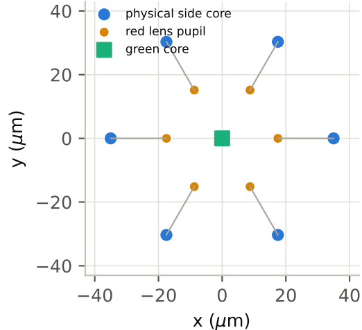
(b) MCF end-face geometry
