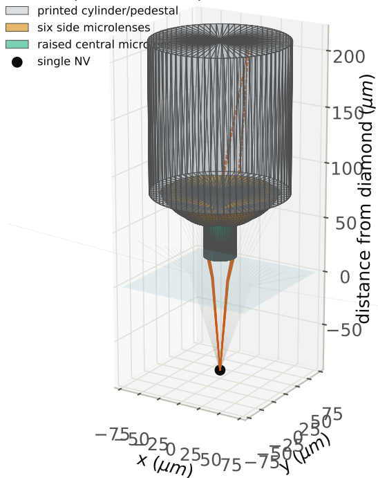
(a) Full printed MCF tip
