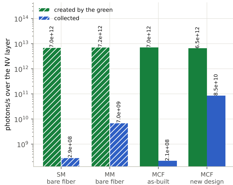
(a) made vs caught, 10 mW green
