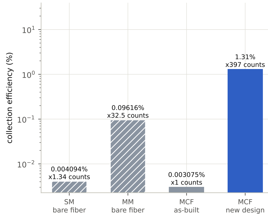
(b) efficiency, and counts against the as-built tip
