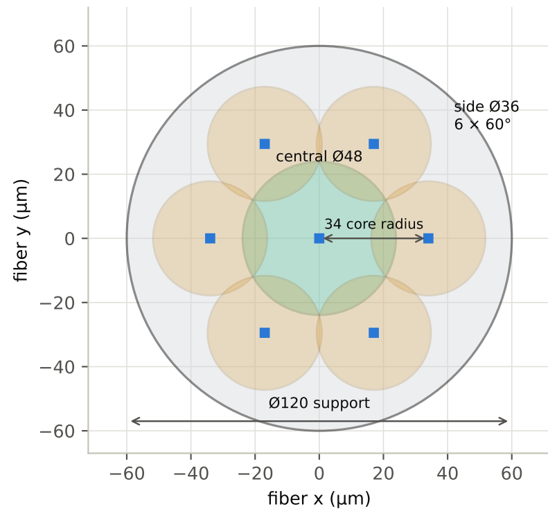
(a) Fiber-facet layout
