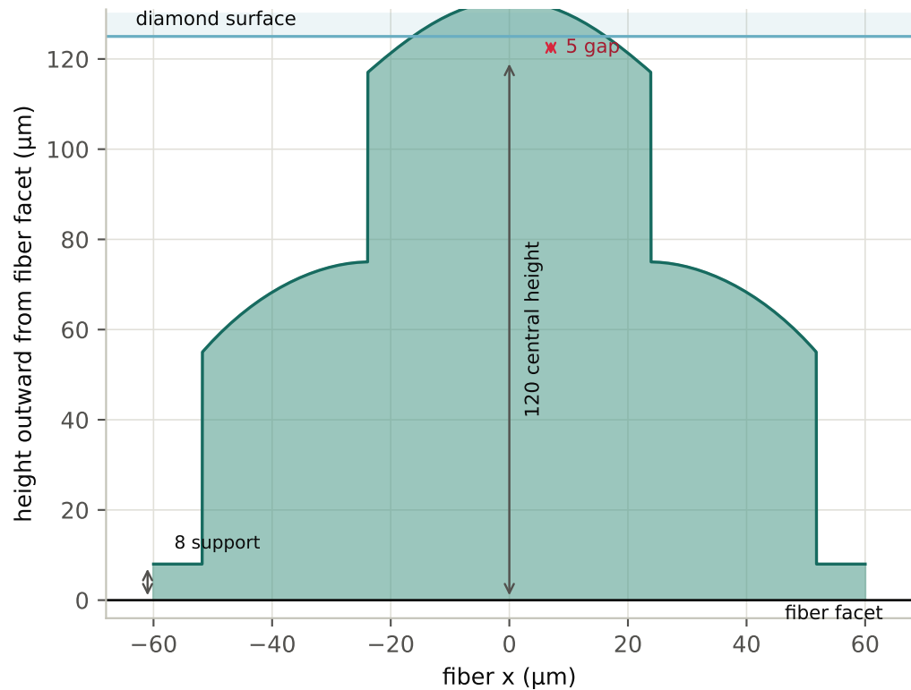
(b) Monolithic x-z section through two side cores
