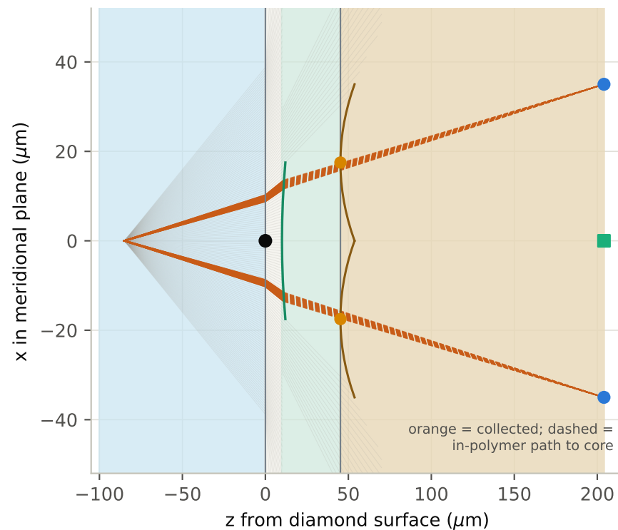
(c) 700 nm rays at fixed-design optimum, g = 10 \mu\text{m}
