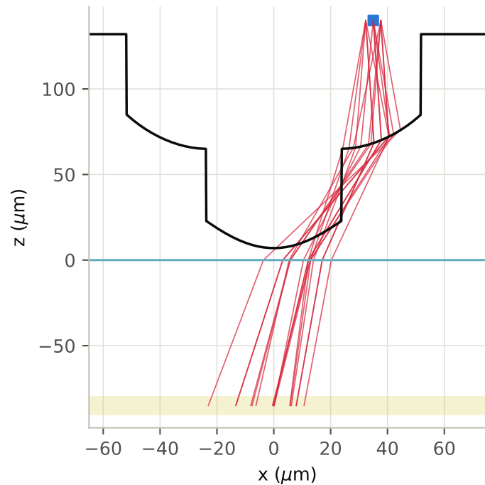
(c) Side-core reciprocal collection, 750 nm
