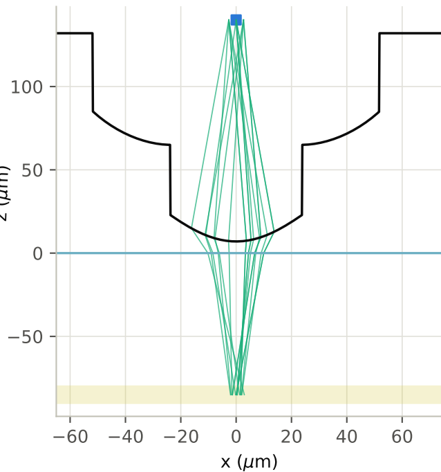
(b) Central excitation, 532 nm
