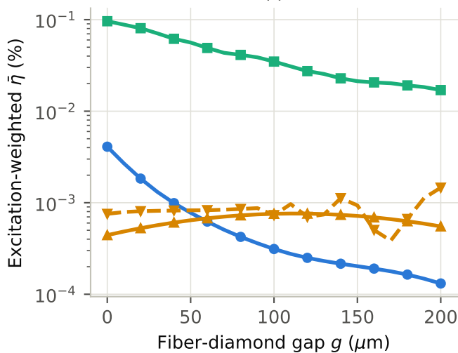
(c) 3D ensemble, 3 ppm
