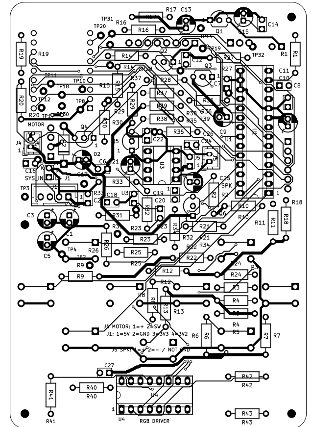
KK MAIN C.4 – REAR FIT CHECK / 80 x 115mm / PROTOTYPE
