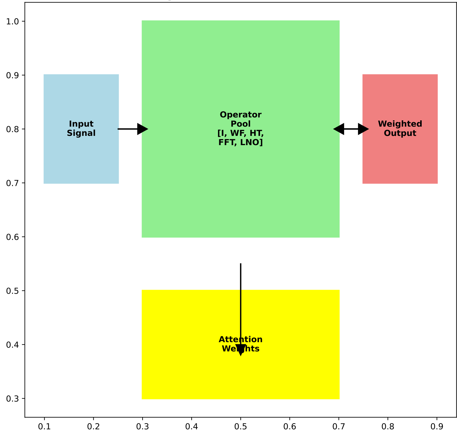
OperatorAttention
