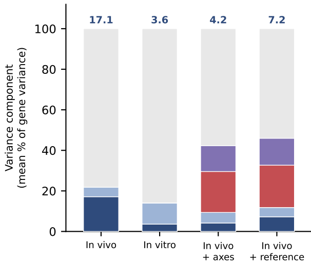
a Variance composition
