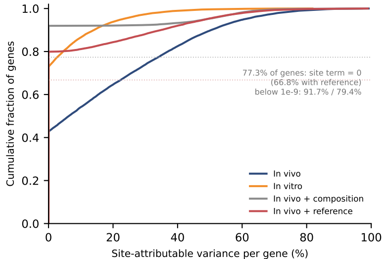
b Site variance per gene
