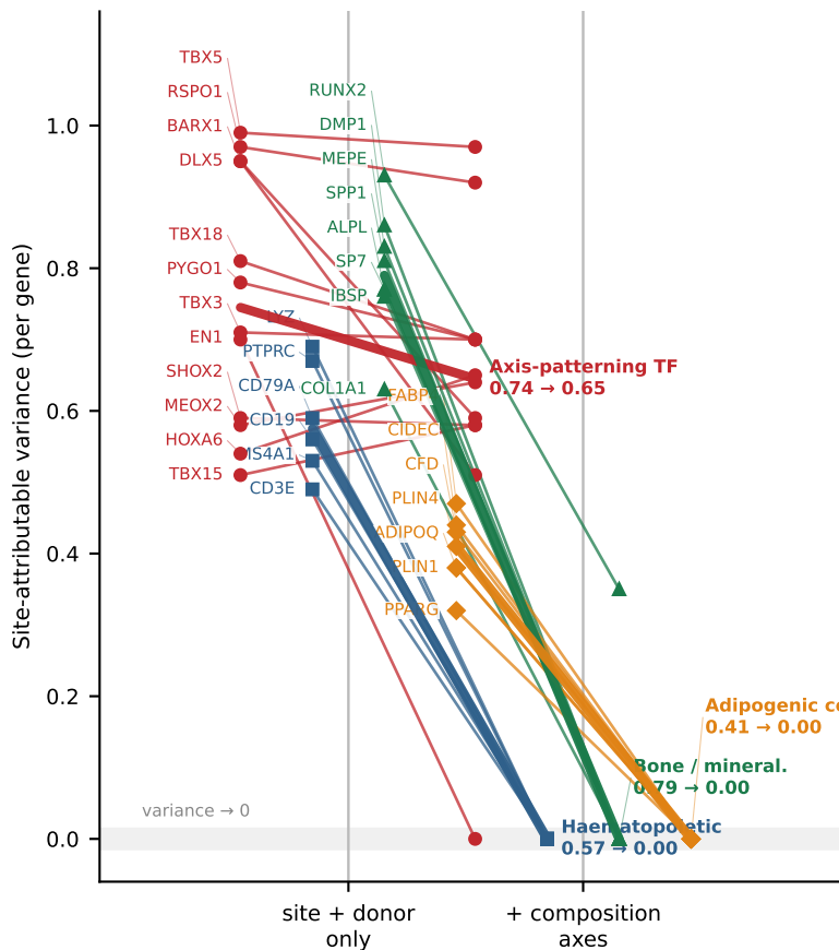
a Positive control: known positional-identity genes survive, composition markers do not
