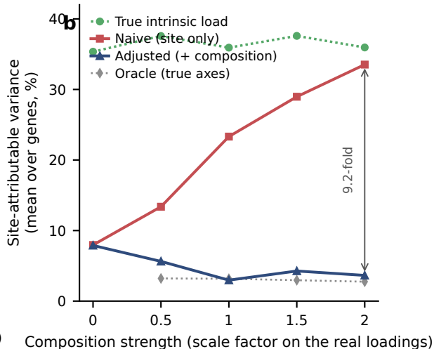
The naive estimate tracks the confounder
