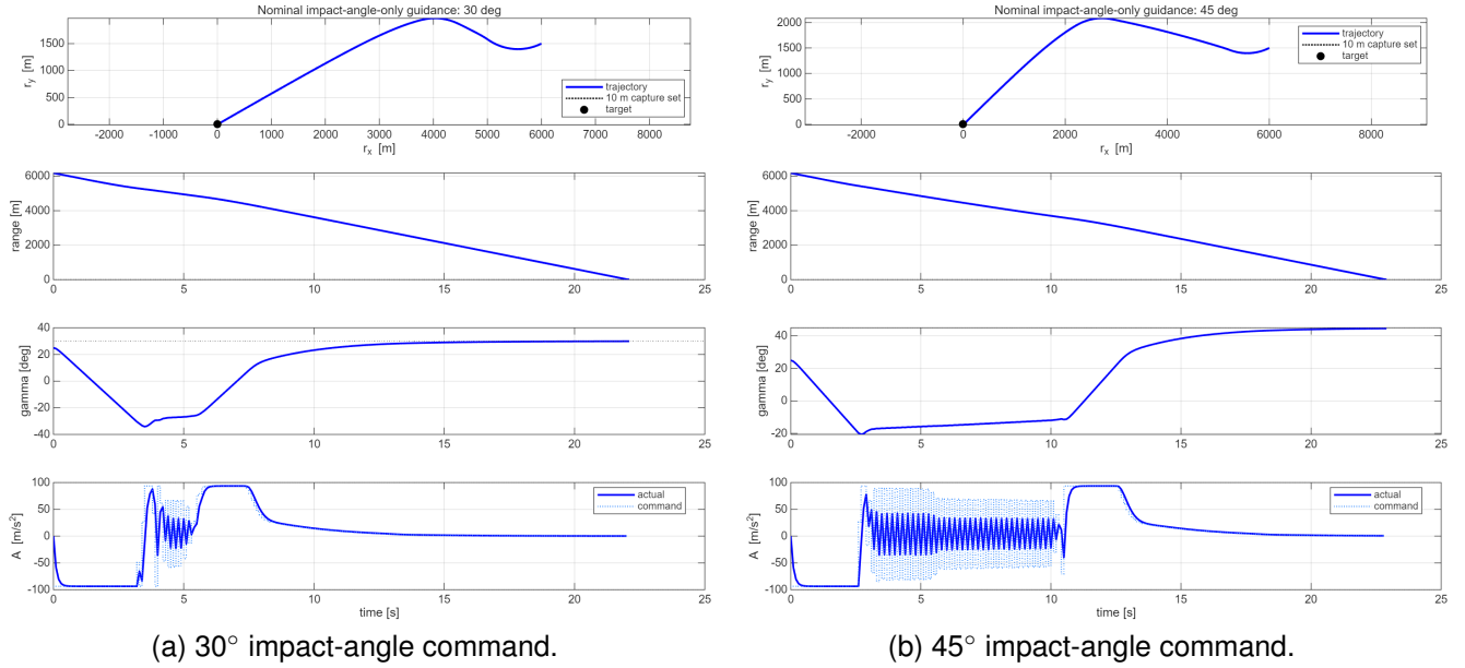
Fig. 3. Nominal flight simulations for the 30° and 45° impact-angle-only cases. Each plot shows the trajectory, range, heading, and first-order-autopilot lateral acceleration.
