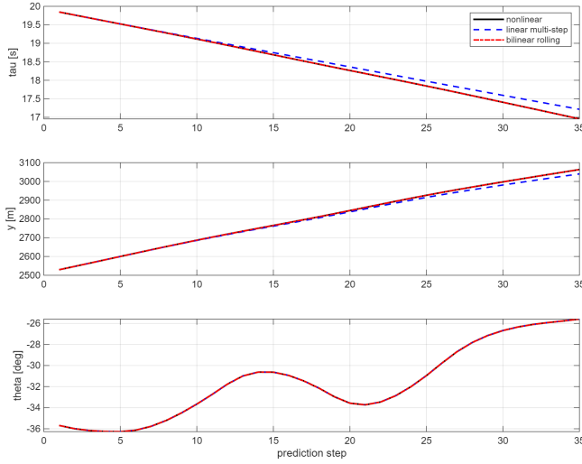
Fig. 1. Prediction comparison between the nonlinear trajectory, the direct linear multi-step EDMD predictor, and the rolling bilinear Koopman predictor.
